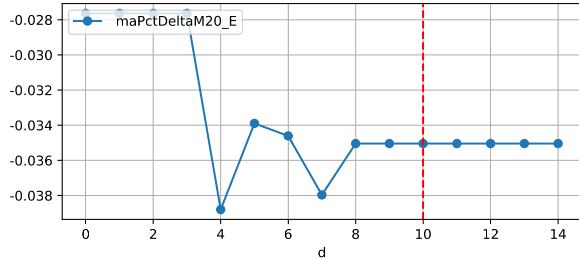
Daily %DeltaM and %DeltaM/1000ml ETcIdef for M20_E (-3.5%/D, -11.2%/1000ml ET)
