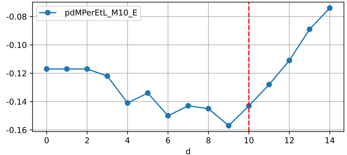
Daily %DeltaM and %DeltaM/1000ml ETcldef for M10_E (-4.5%/D, -14.3%/1000ml ET)
