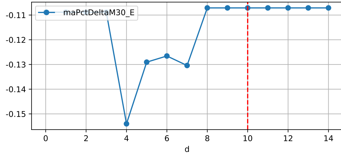
Daily %DeltaM and %DeltaM/1000ml ETcIdef for M30_E (-10.7%/D, -34.2%/1000ml ET)
