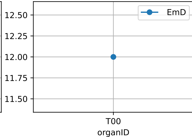
EQ2AE (Raw data plots) EQ2AE-24-33 Phe
