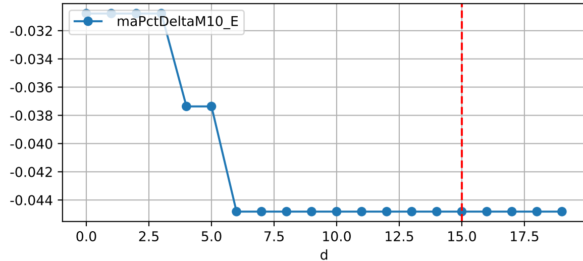
Daily %DeltaM and %DeltaM/1000ml ETcIdef for M10_E (-4.5%/D, -8.2%/1000ml ET)
