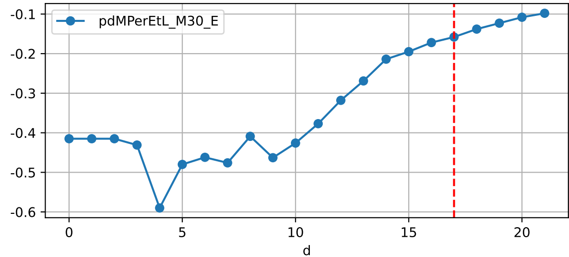
Daily %DeltaM and %DeltaM/1000ml ETcIdef for M30_E (-10.7%/D, -15.8%/1000ml ET)
