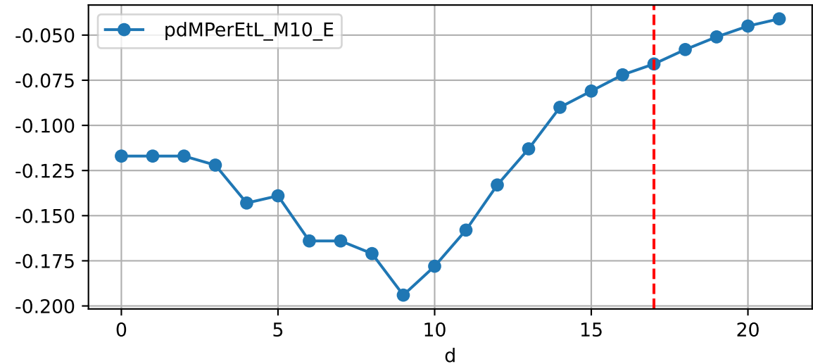
Daily %DeltaM and %DeltaM/1000ml ETcIdef for M10_E (-4.5%/D, -6.6%/1000ml ET)
