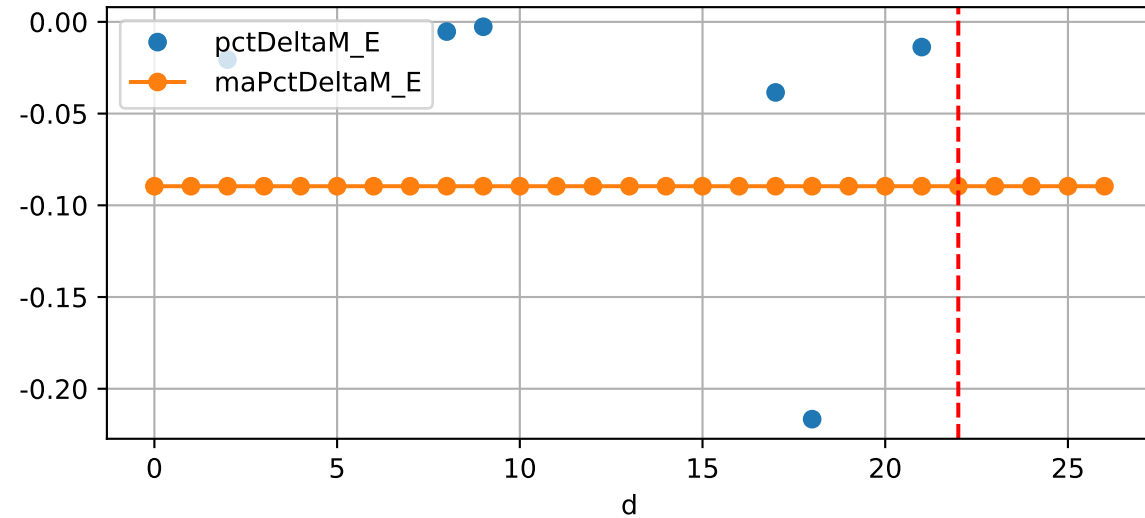
Daily %DeltaM and %DeltaM/1000ml ETcldef for M_E (-9.0%/D, -15.0%/1000ml ET)
