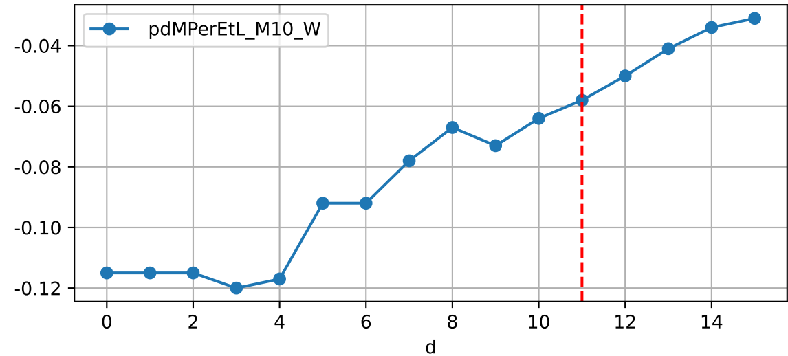
Daily %DeltaM and %DeltaM/1000ml ETcldef for M10_W (-2.1%/D, -5.8%/1000ml ET)
