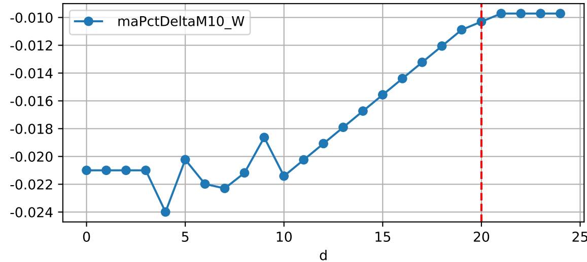
Daily %DeltaM and %DeltaM/1000ml ETcldef for M10_W (-1.0%/D, -1.4%/1000ml ET)
