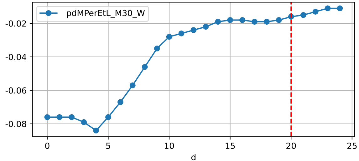
Daily %DeltaM and %DeltaM/1000ml ETcIdef for M30_W (-1.2%/D, -1.6%/1000ml ET)
