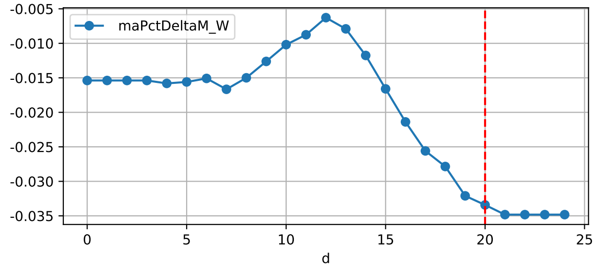
Daily %DeltaM and %DeltaM/1000ml ETcIdef for M_W (-3.3%/D, -4.5%/1000ml ET)
