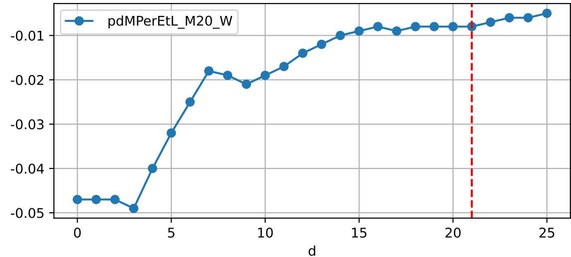
Daily %DeltaM and %DeltaM/1000ml ETcldef for M20_W (-0.4%/D, -0.8%/1000ml ET)
