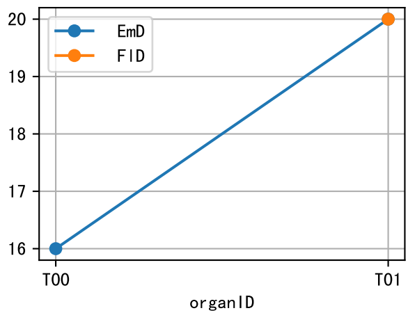
EQ2AWavg Phe
