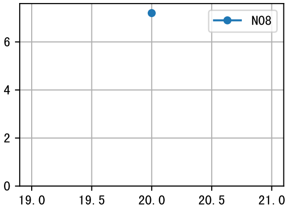
NdD (EQ2AW-49-6)
