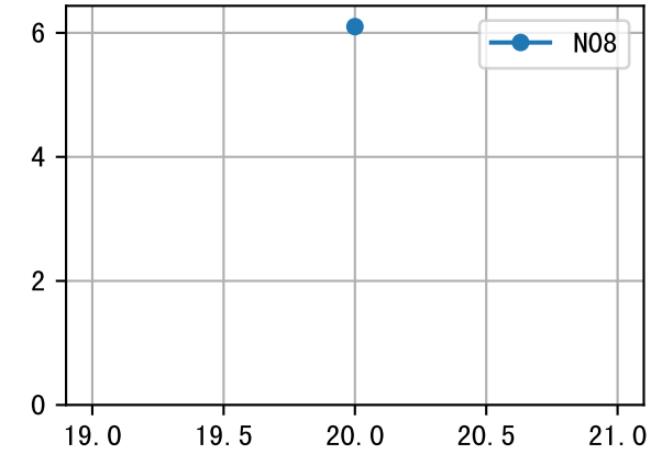
NdD (EQ2AW-41-47)
