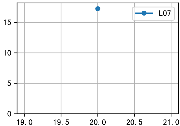
LfW (EQ2AWavg)
