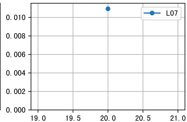
LfA (EQ2AWavg)
