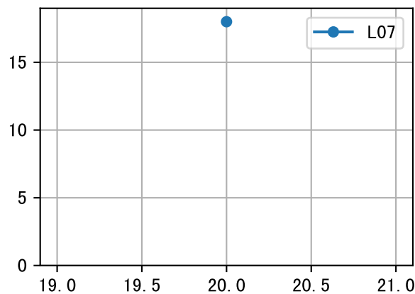
LfL (EQ2AW-32-58)
