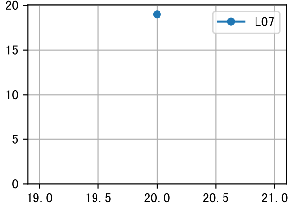
LfL (EQ2AW-38-31)
