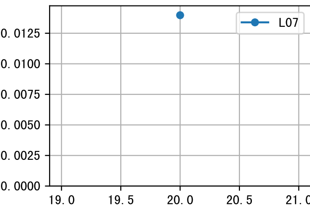
LfA (EQ2AW-49-6)
