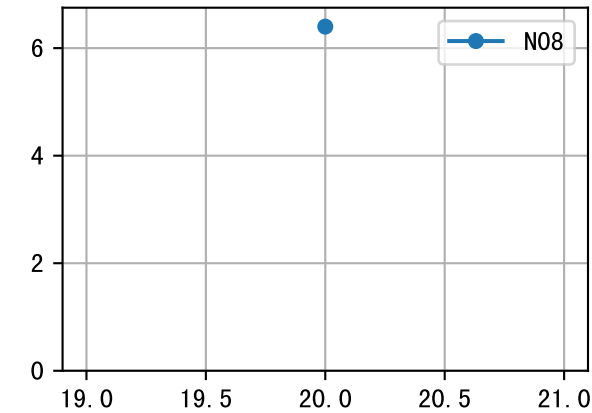
NdD (EQ2AW-38-31)
