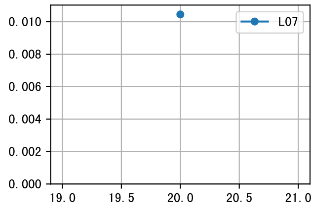
LfA (EQ2AW-38-31)
