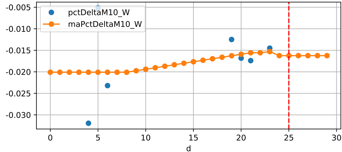
Daily %DeltaM and %DeltaM/1000ml ETcIdef for M10_W (-1.6%/D, -6.2%/1000ml ET)
