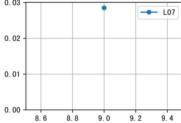
LfA (EQ4AW-42-9) Plot By Age
