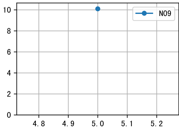
NdD (EQ4AW-38-23) Plot By Age
