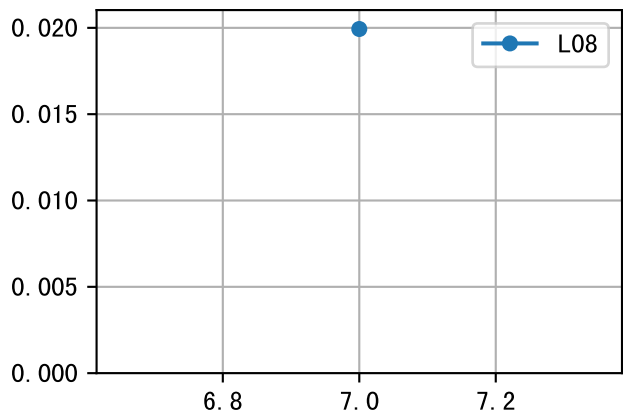
LfA (EQ4AW-38-23) Plot By Age
