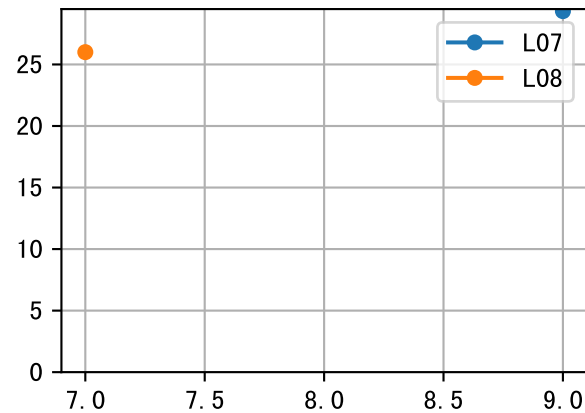
LfL (EQ4AWavg) Plot By Age
