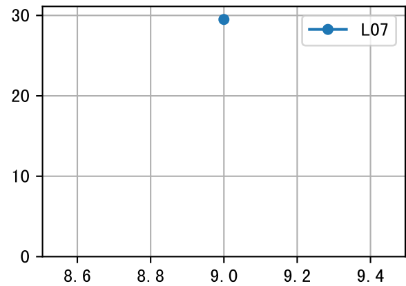
LfL (EQ4AW-27-18) Plot By Age
