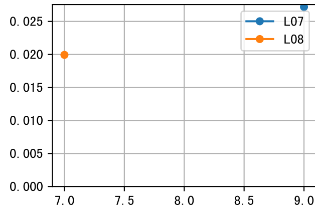
LfA (EQ4AWavg) Plot By Age
