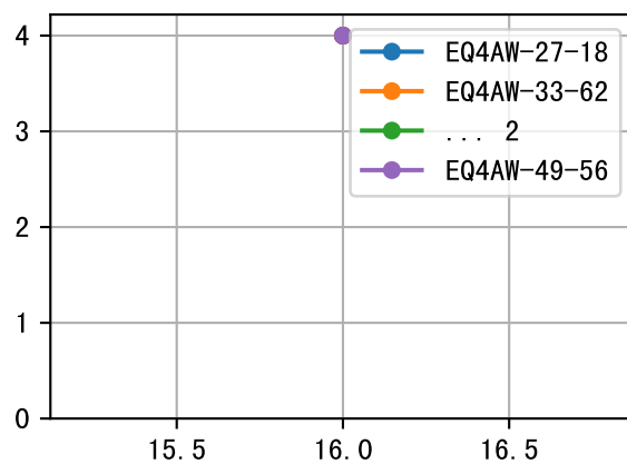
EQ4AW (Raw data plots)
