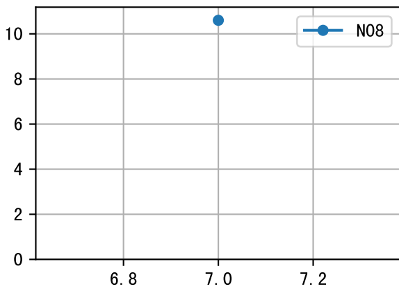
NdD (EQ4AW-49-56) Plot By Age
