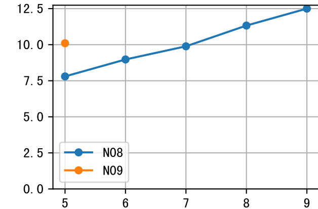
NdD (EQ4AWavg) Plot By Age
