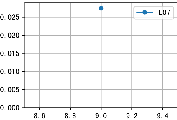
LfA (EQ4AW-49-56) Plot By Age
