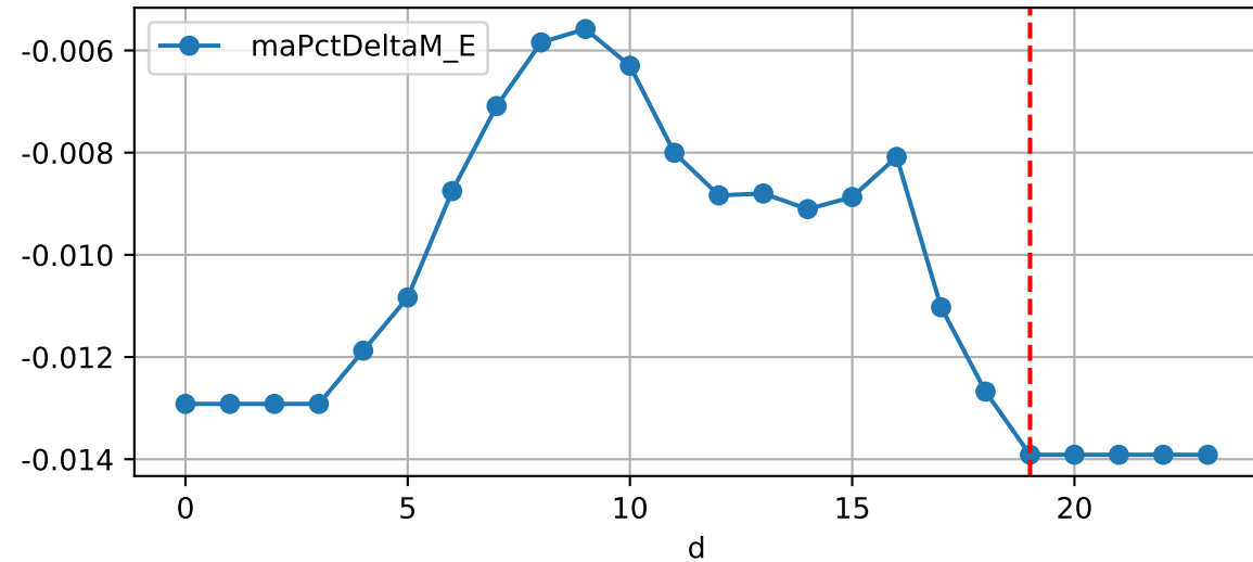
Daily %DeltaM and %DeltaM/1000ml ETcldef for M_E (-1.4%/D, -2.0%/1000ml ET)
