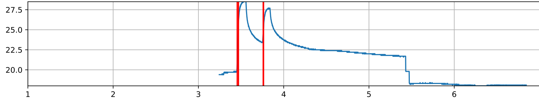
G3-10_0: M_W
