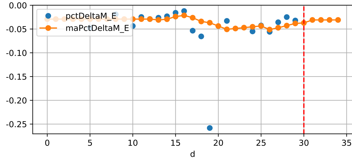
Daily %DeltaM and %DeltaM/1000ml ETcldef for M_E (-3.7%/D, -3.4%/1000ml ET)
