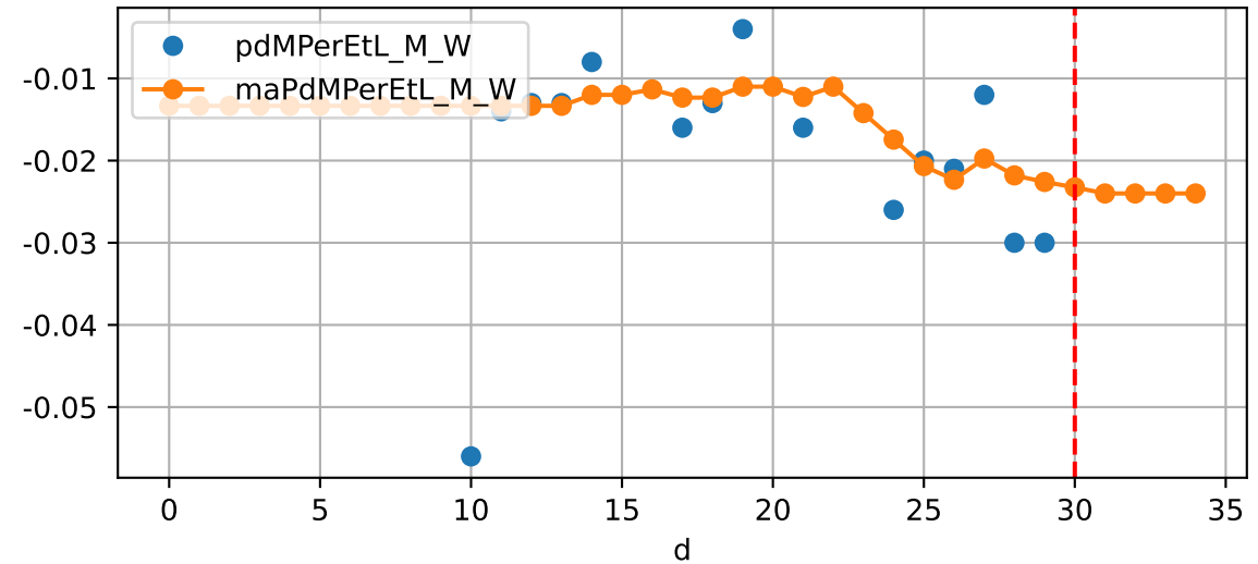
Daily %DeltaM and %DeltaM/1000ml ETcIdef for M_W (-2.5%/D, -2.3%/1000ml ET)
