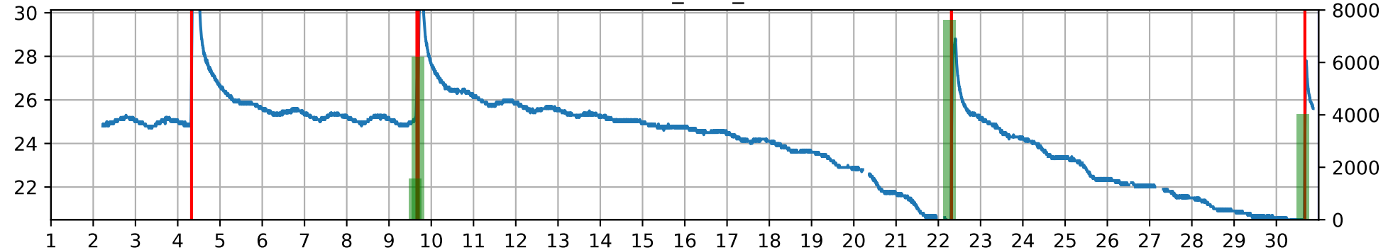
G3-13_0: M_W
