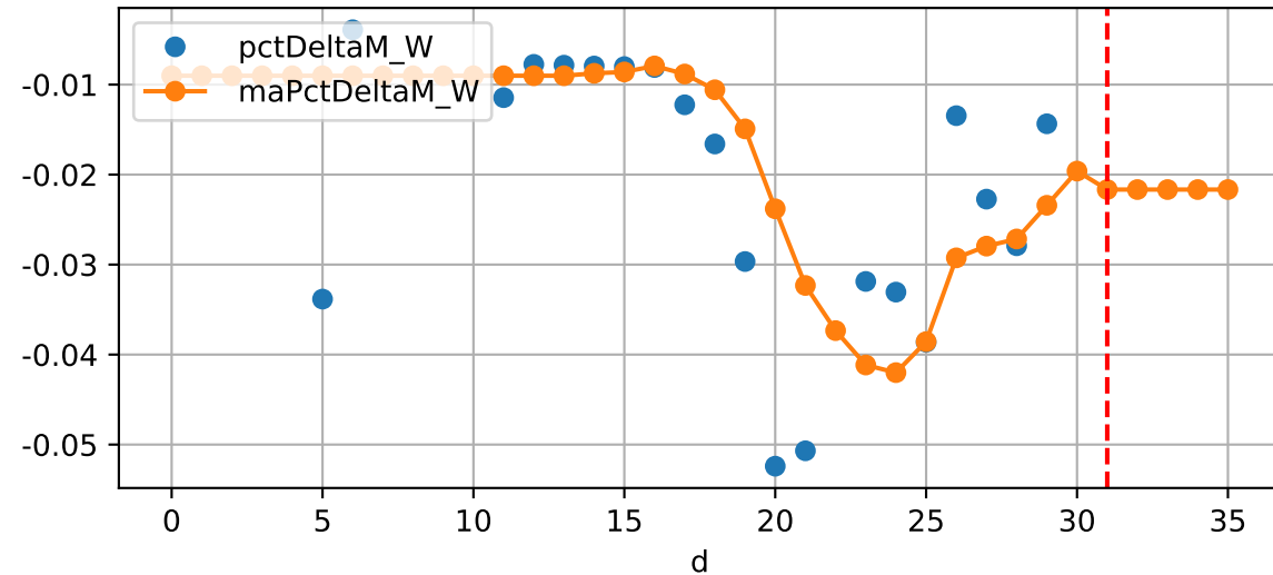
Daily %DeltaM and %DeltaM/1000ml ETcIdef for M_W (-2.2%/D, -3.0%/1000ml ET)
