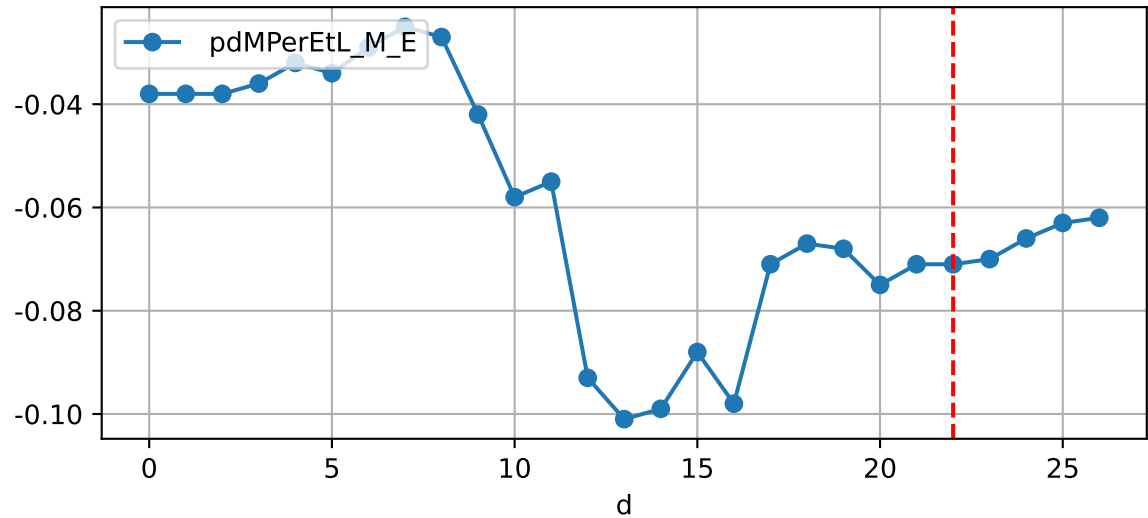
Daily %DeltaM and %DeltaM/1000ml ETcldef for M_E (-8.4%/D, -7.1%/1000ml ET)
