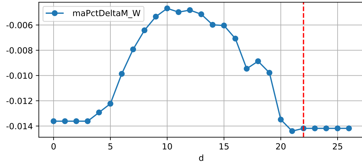
Daily %DeltaM and %DeltaM/1000ml ETcIdef for M_W (-1.4%/D, -1.2%/1000ml ET)
