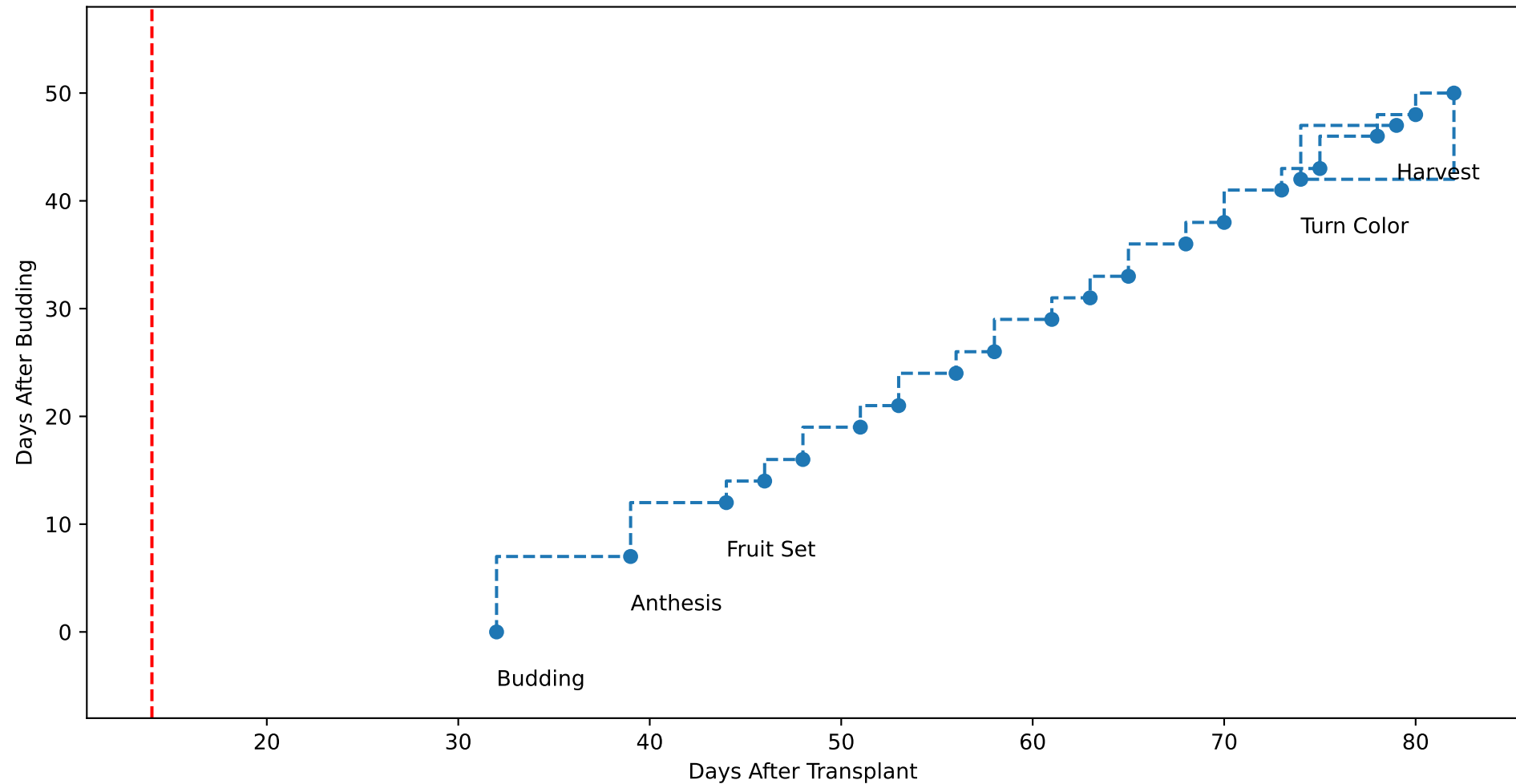
G3-15 TsN4 (plot by DAT)
