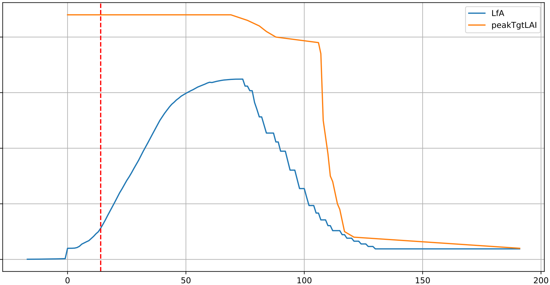
G3-15: ['LfA', 'peakTgtLAI']
