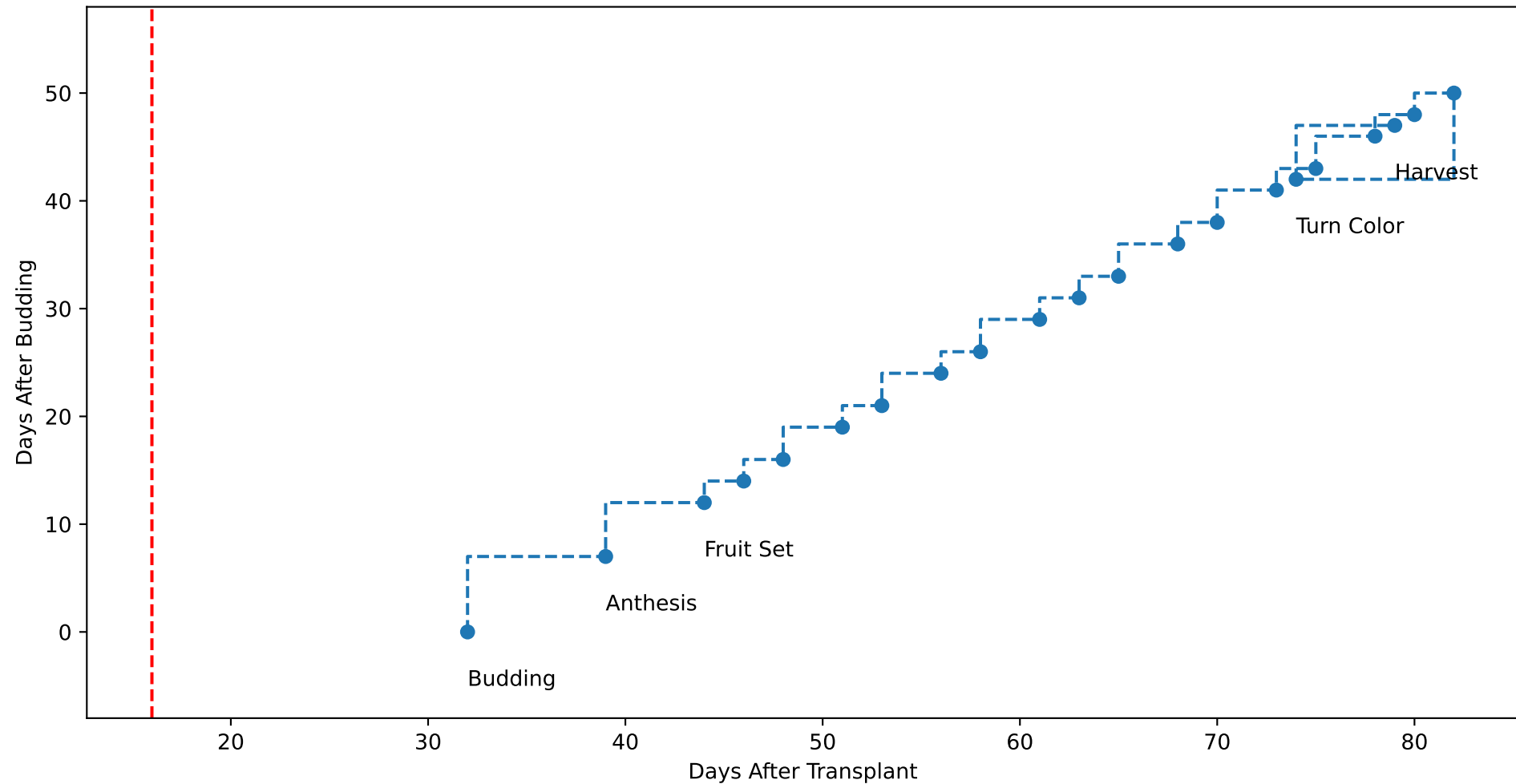
G3-15 TsN4 (plot by adjDAT)
