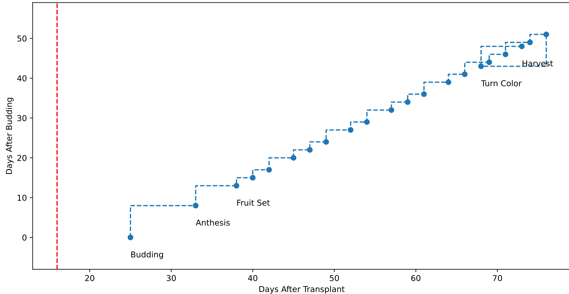
G3-15 TsN3 (plot by adjDAT)
