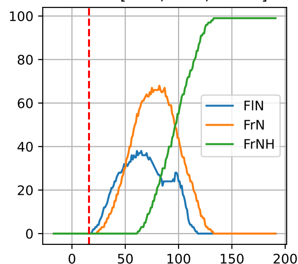
G3-15: ['FIN', 'FrN', 'FrNH']
