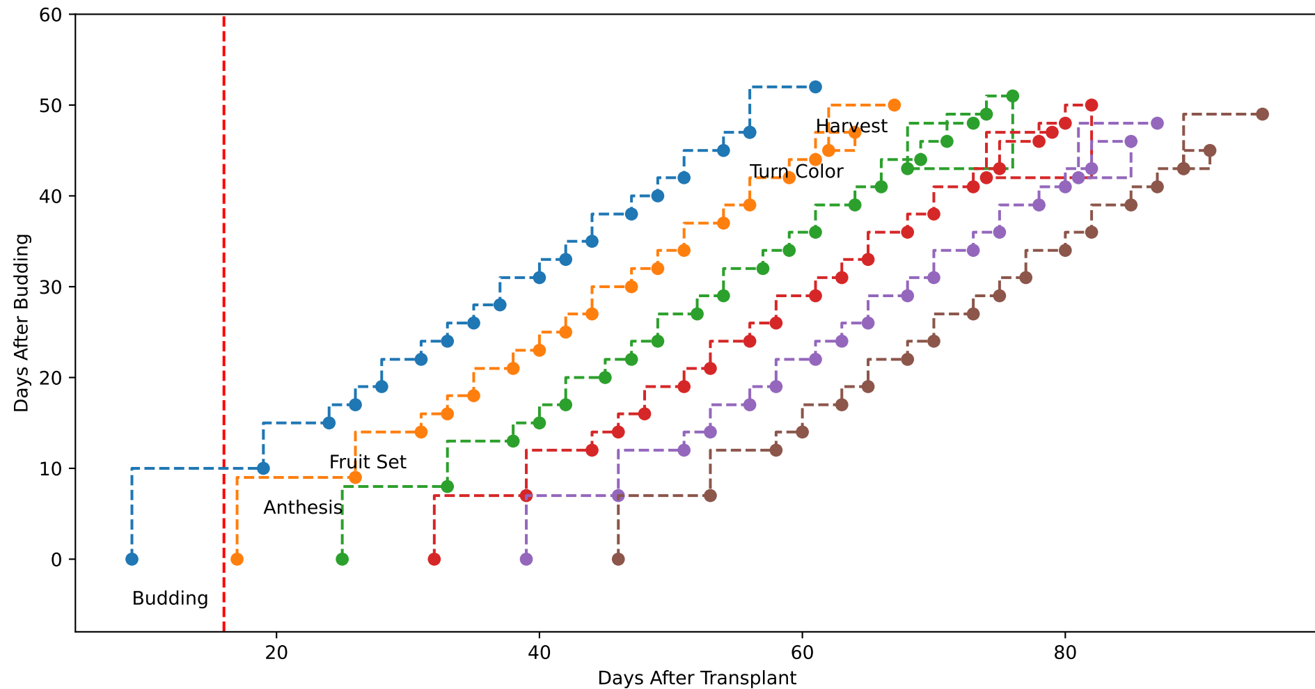
G3-15 (plot by DAT)
