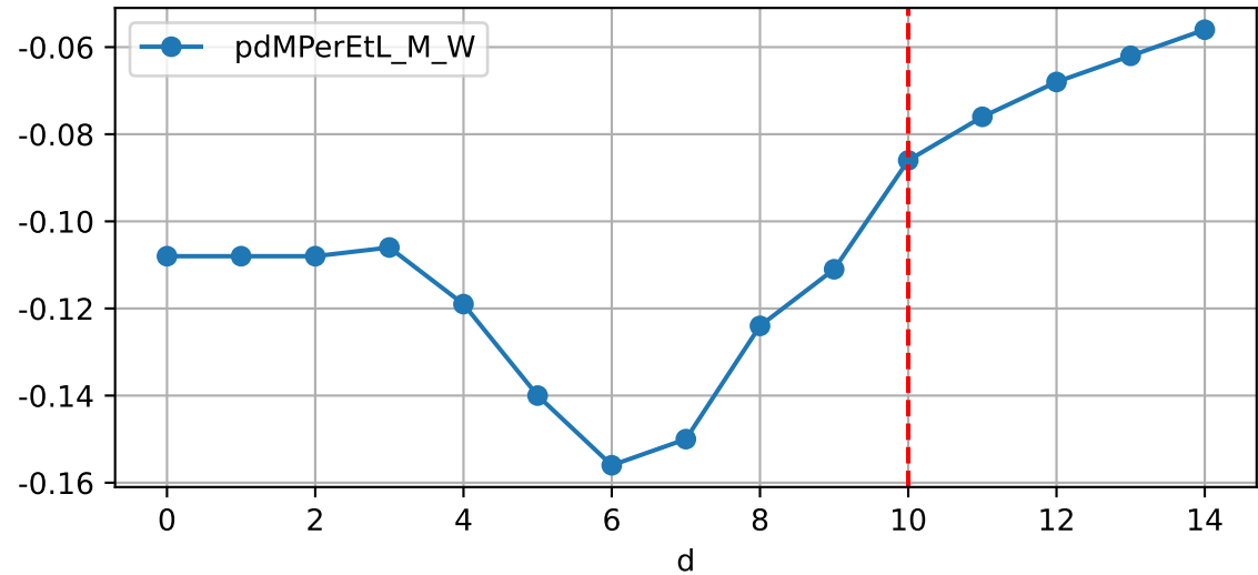
Daily %DeltaM and %DeltaM/1000ml ETcIdef for M_W (-3.8%/D, -8.6%/1000ml ET)
