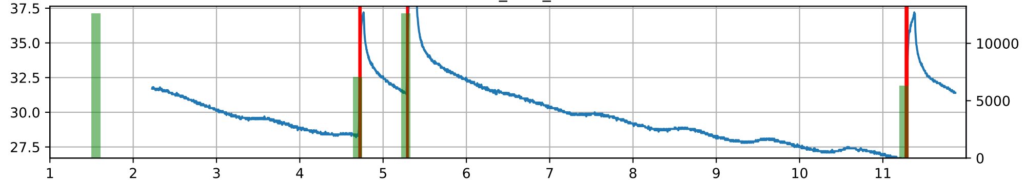
G3-17_0: M_W
