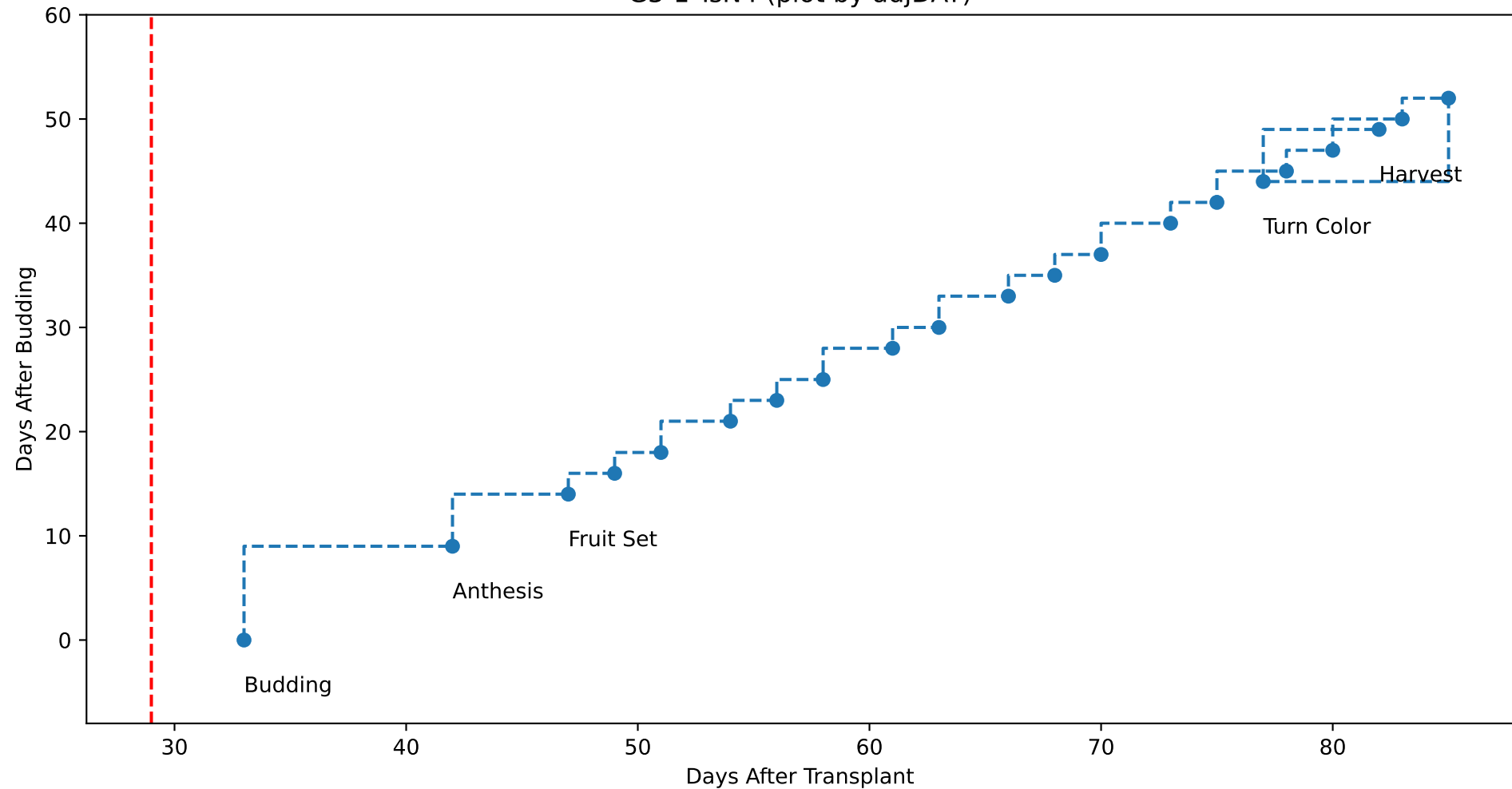
G3-1 TsN4 (plot by adjDAT)
