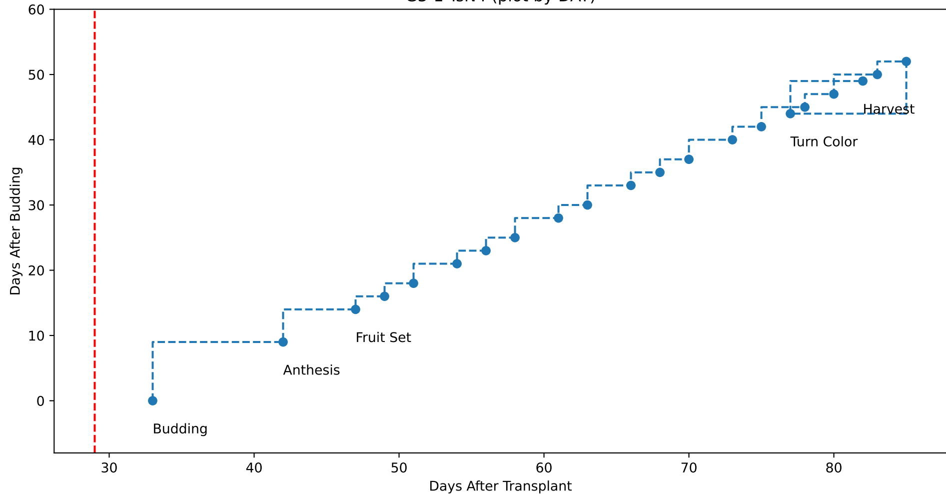
G3-1 TsN4 (plot by DAT)
