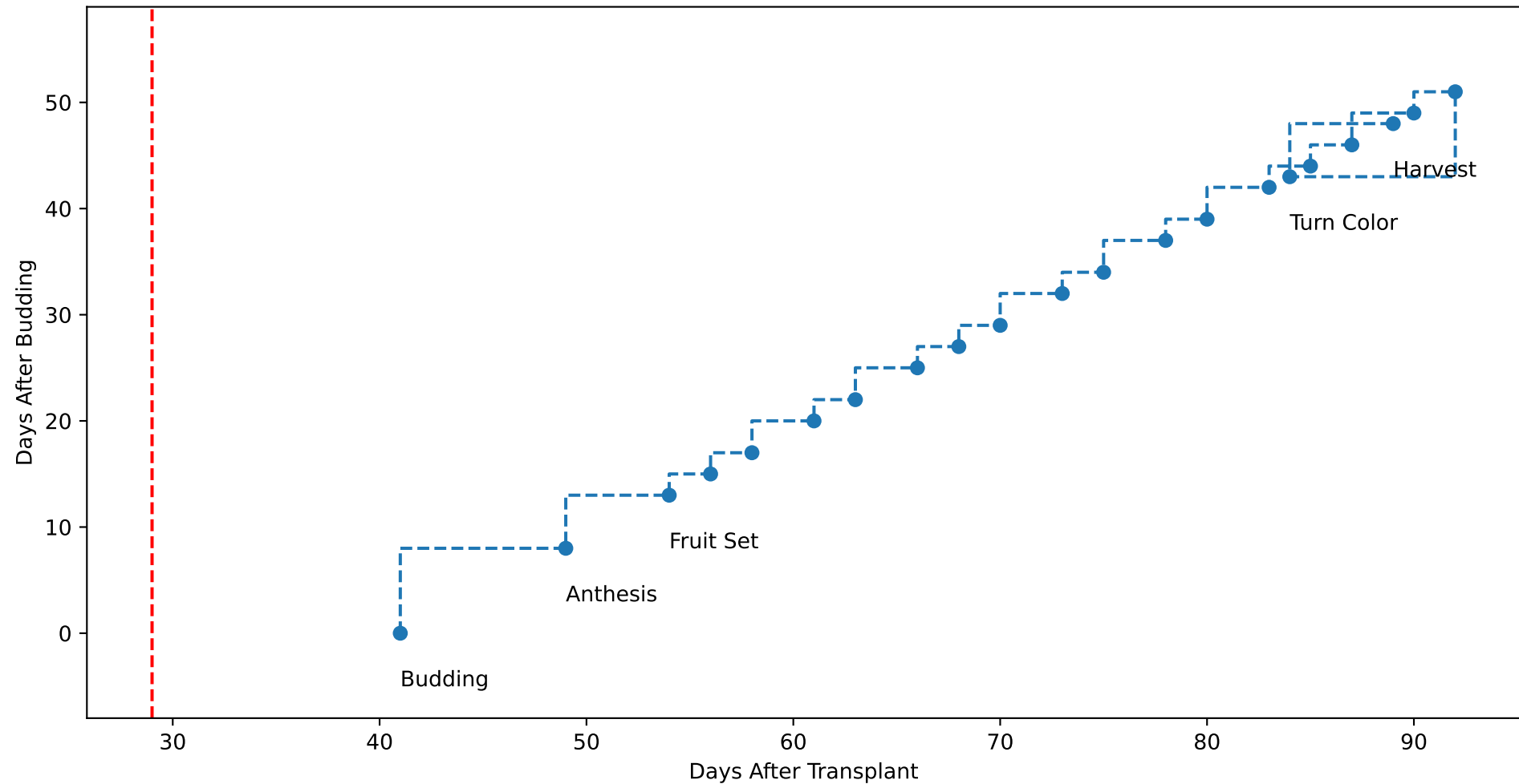
G3-1 TsN5 (plot by adjDAT)
