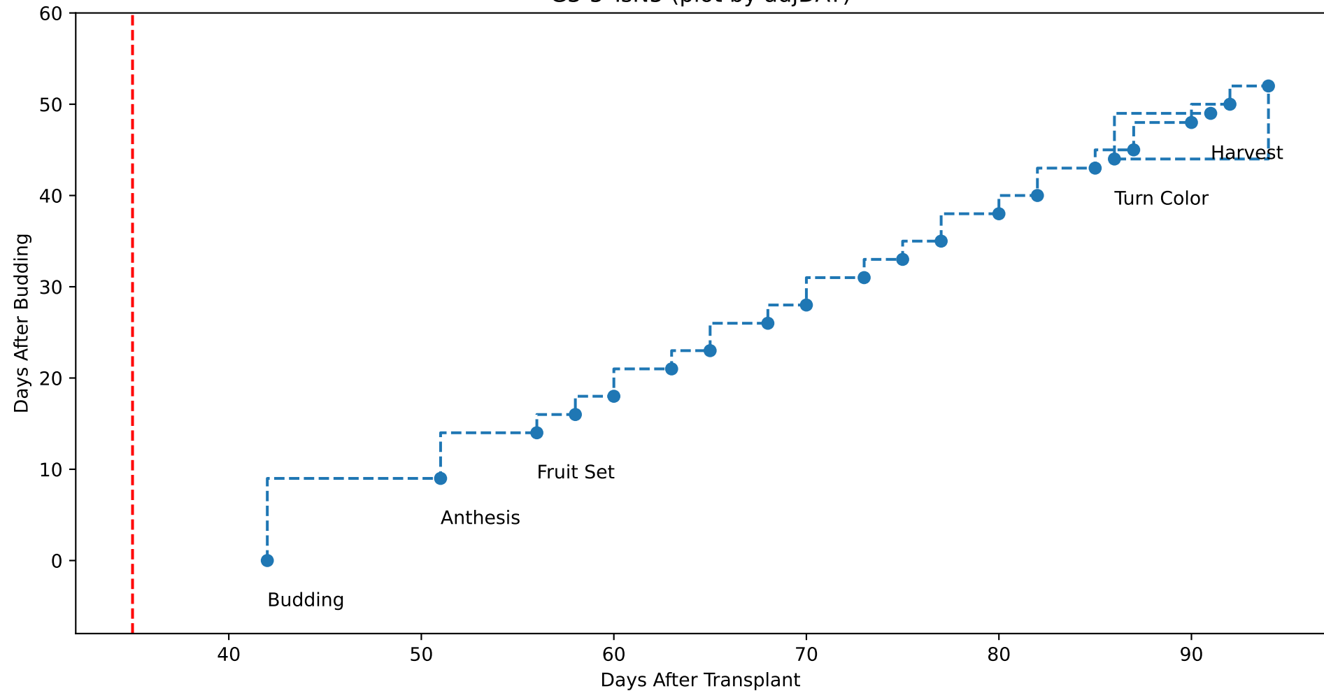
G3-5 TsN5 (plot by adjDAT)
