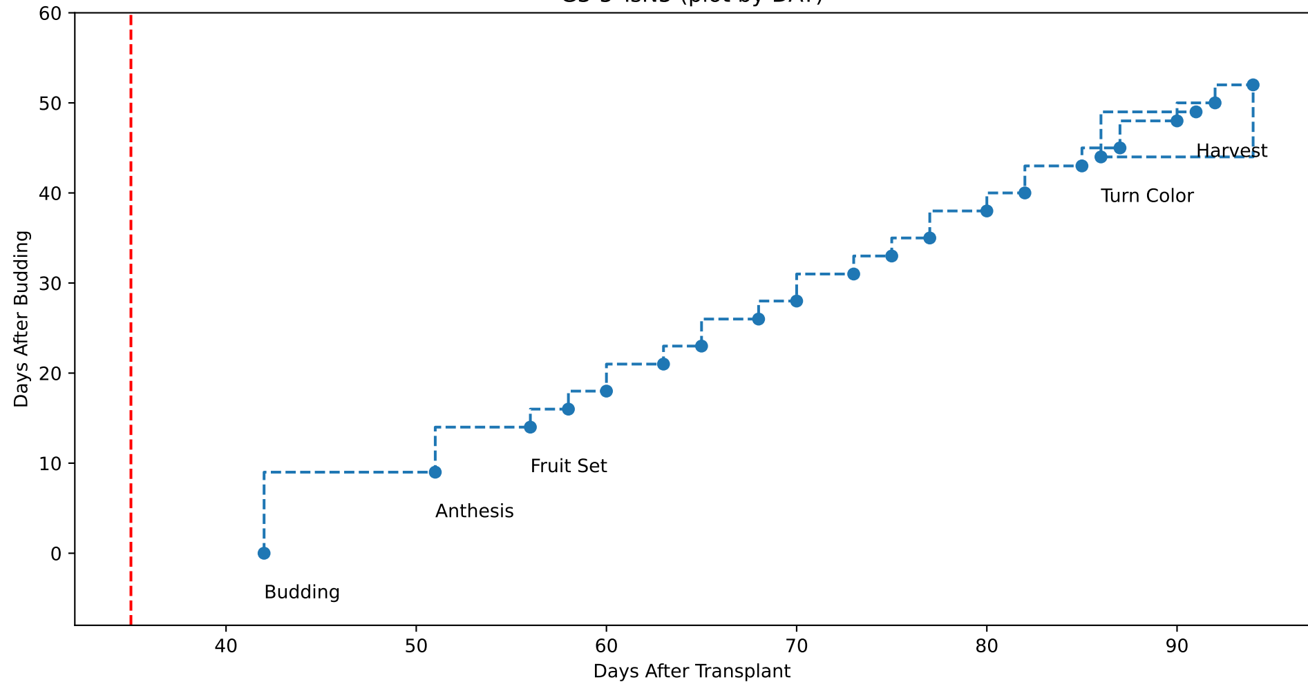
G3-5 TsN5 (plot by DAT)
