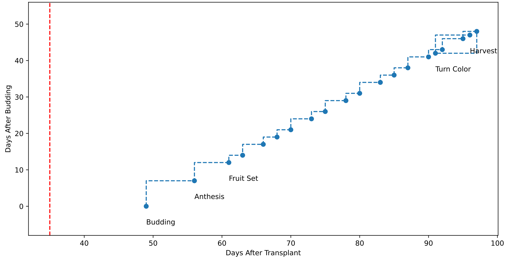
G3-5 TsN6 (plot by adjDAT)
