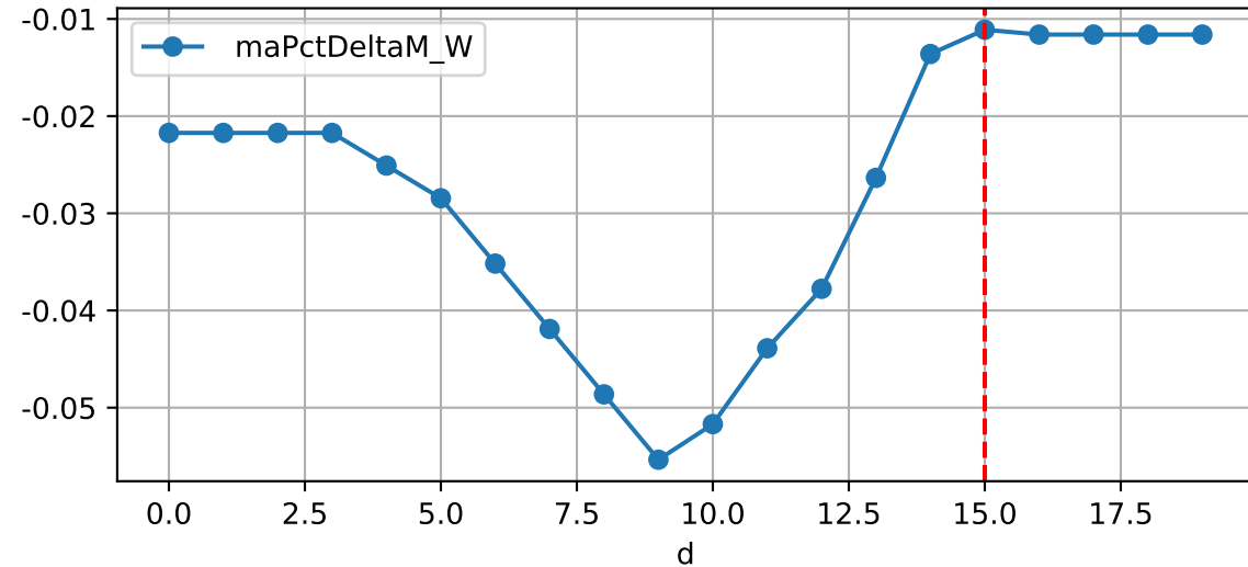
Daily %DeltaM and %DeltaM/1000ml ETcIdef for M_W (-1.1%/D, -1.7%/1000ml ET)
