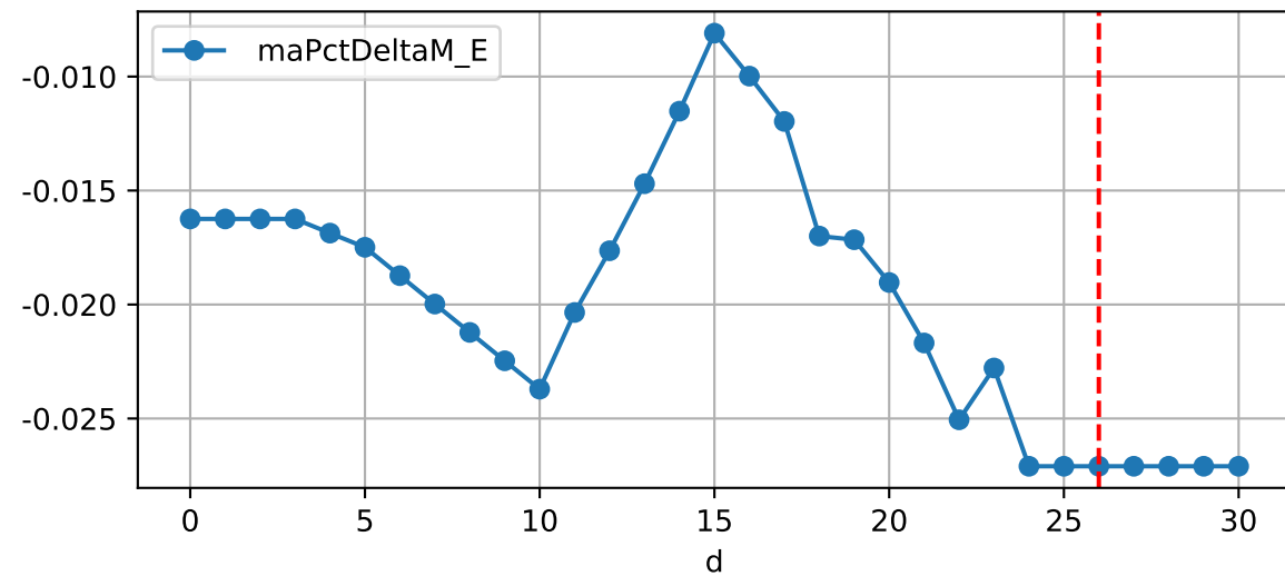
Daily %DeltaM and %DeltaM/1000ml ETcldef for M_E (-2.7%/D, -2.0%/1000ml ET)
