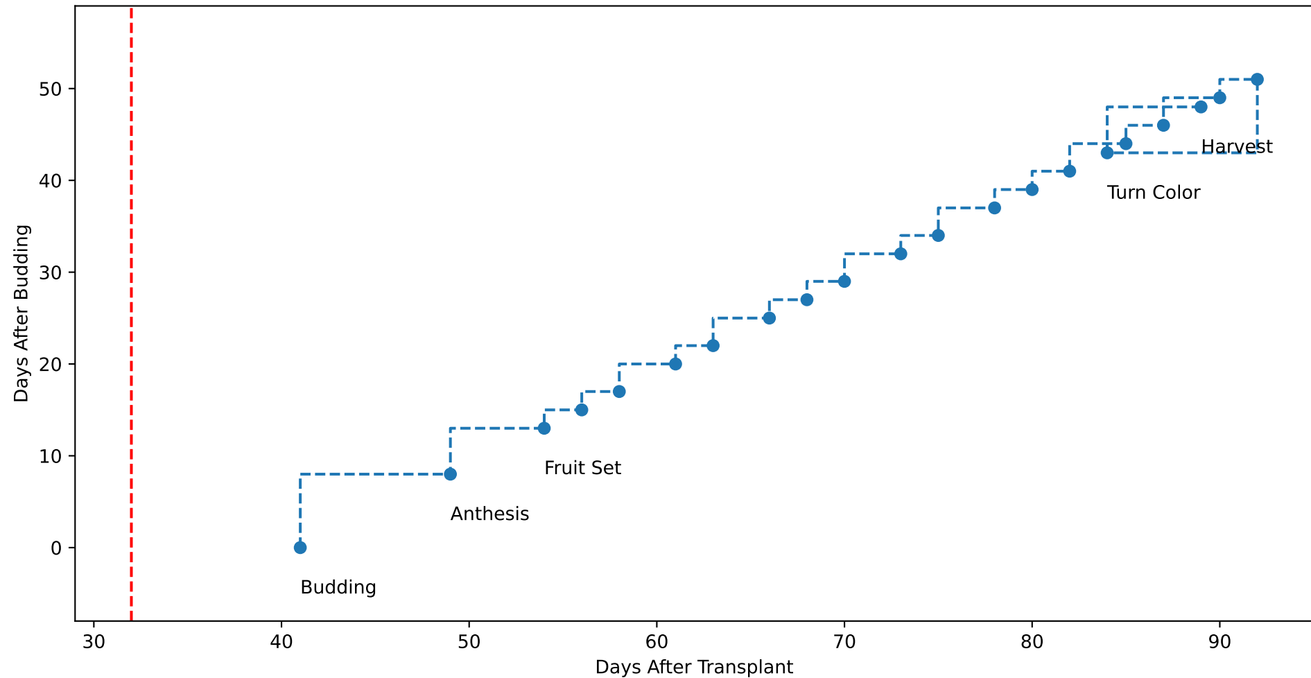
G3-6 TsN5 (plot by adjDAT)
