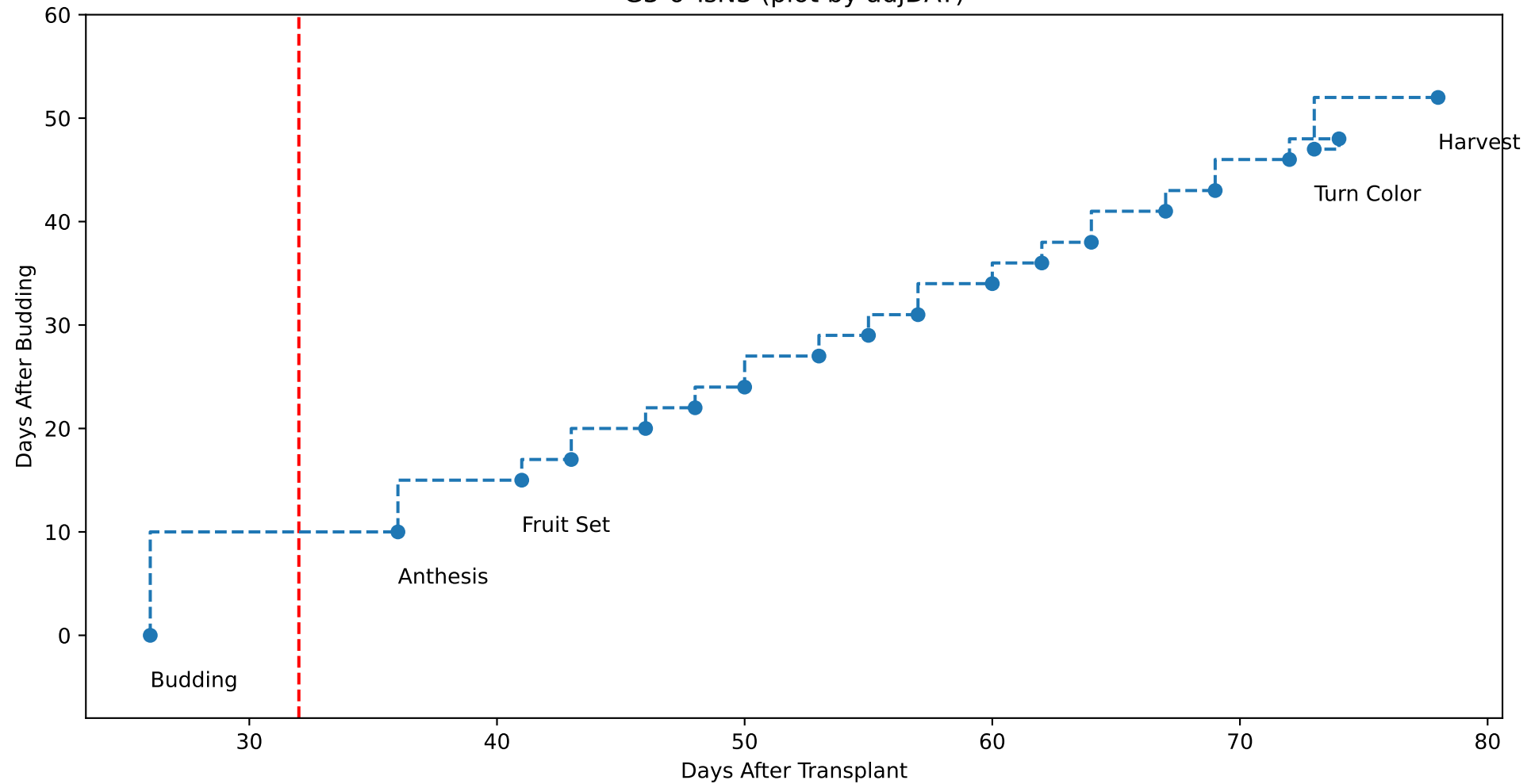
G3-6 TsN3 (plot by adjDAT)
