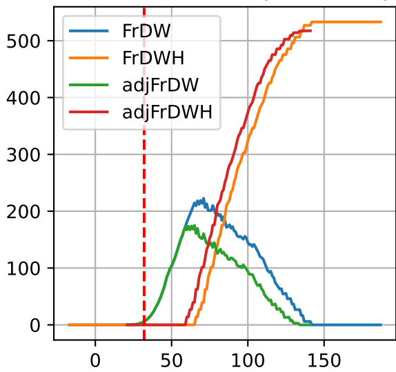
G3-6: ['FrDW', 'FrDWH', 'adjFrDW', 'adjFrDWH']
