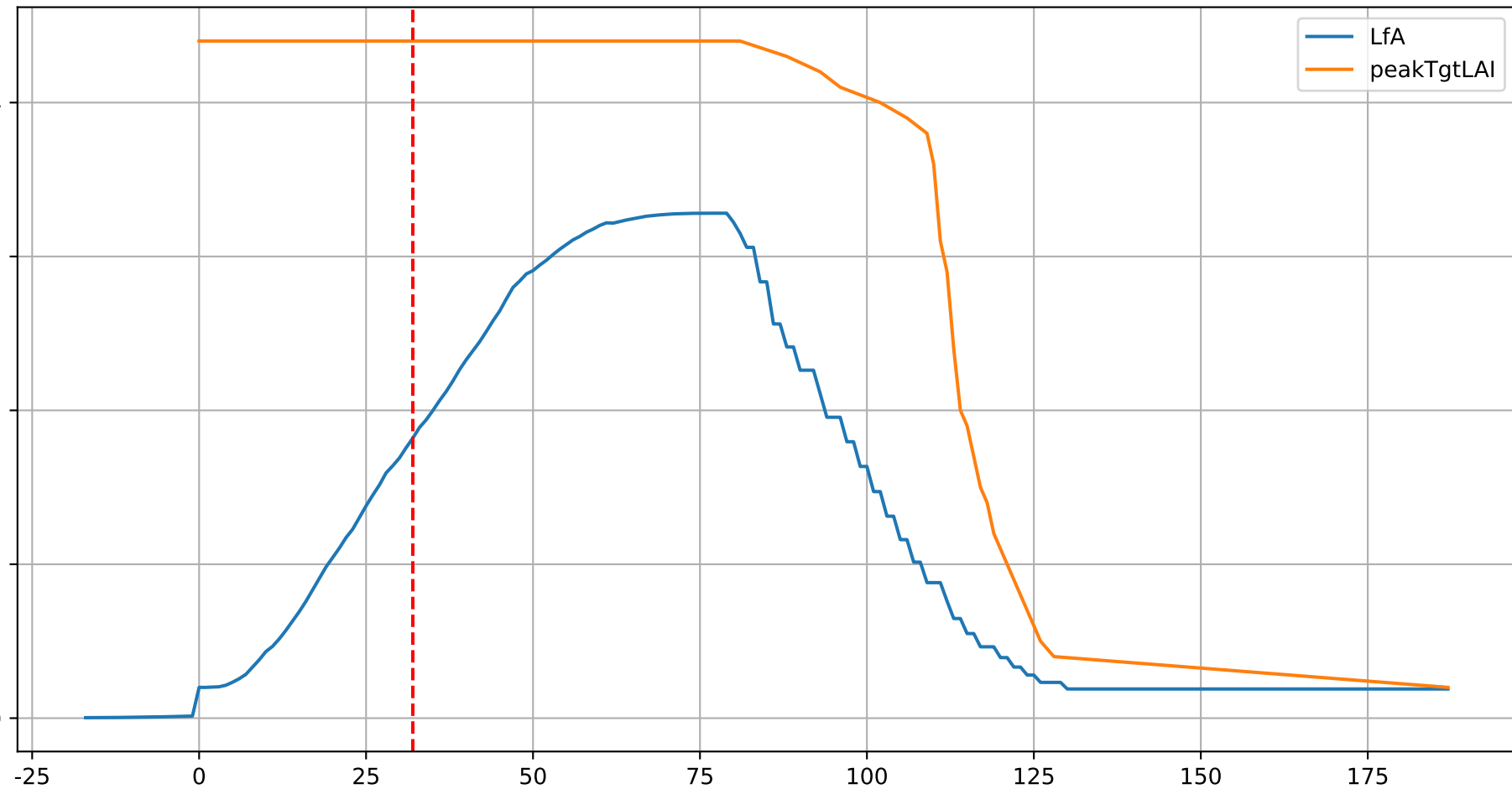
G3-6: ['LfA', 'peakTgtLAI']
