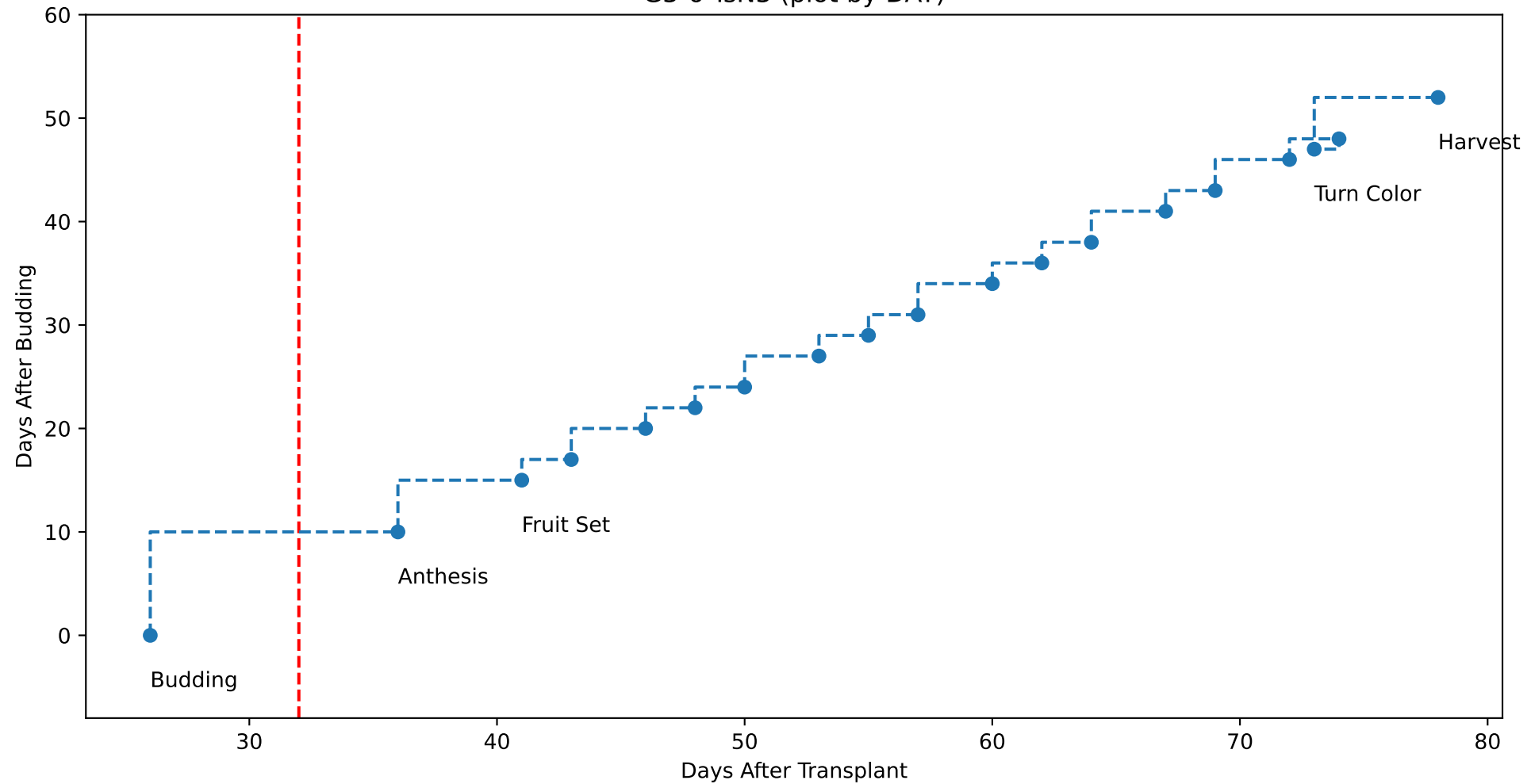
G3-6 TsN3 (plot by DAT)
