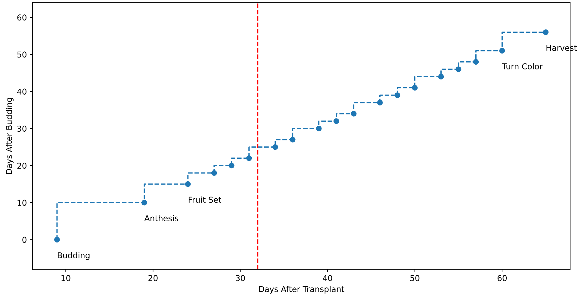
G3-6 TsN1 (plot by DAT)
