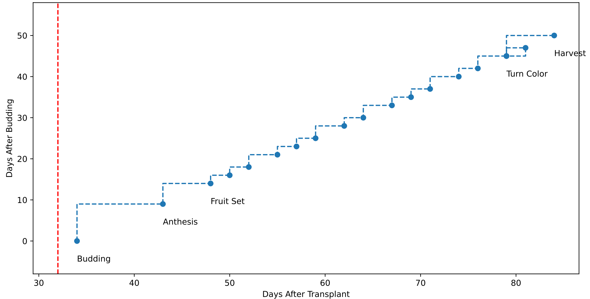
G3-6 TsN4 (plot by adjDAT)
