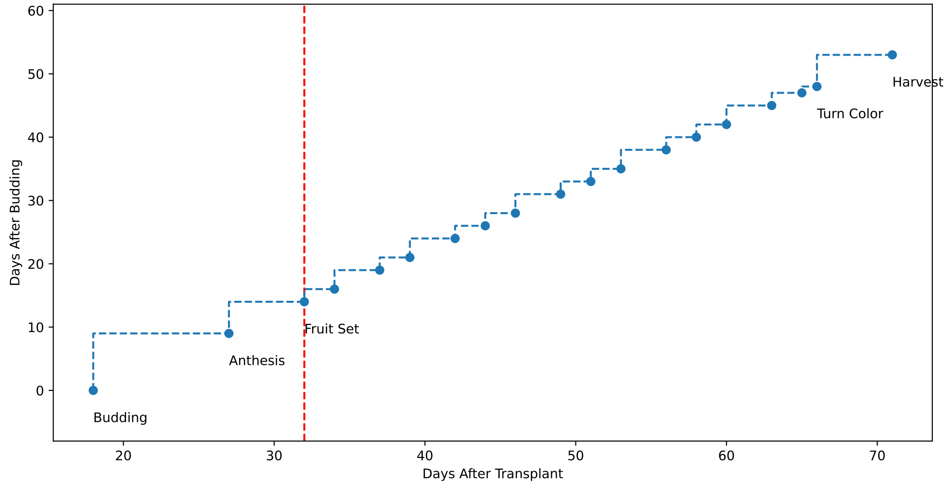
G3-6 TsN2 (plot by adjDAT)
