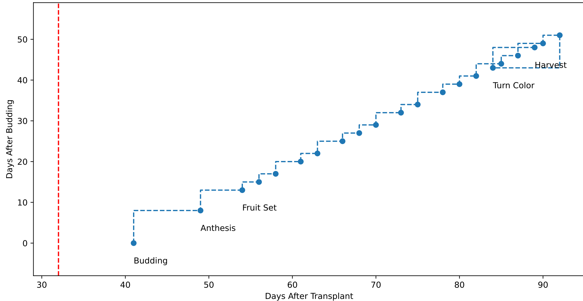
G3-6 TsN5 (plot by DAT)
