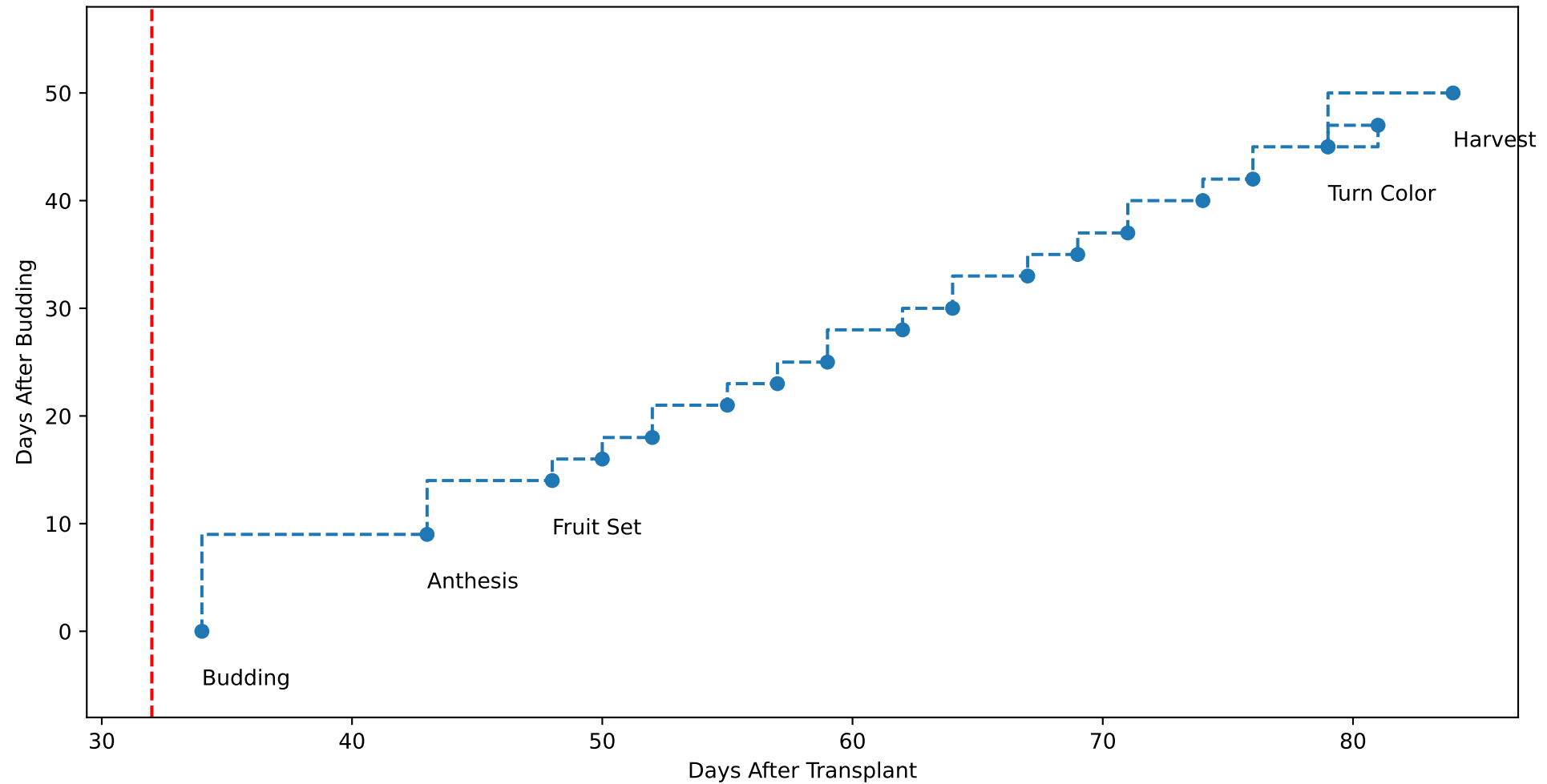
G3-6 TsN4 (plot by DAT)
