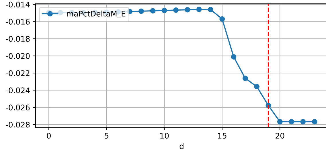
Daily %DeltaM and %DeltaM/1000ml ETcldef for M_E (-2.6%/D, -2.6%/1000ml ET)
