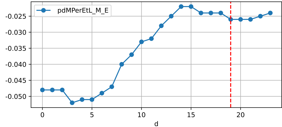
Daily %DeltaM and %DeltaM/1000ml ETcldef for M_E (-2.6%/D, -2.6%/1000ml ET)
