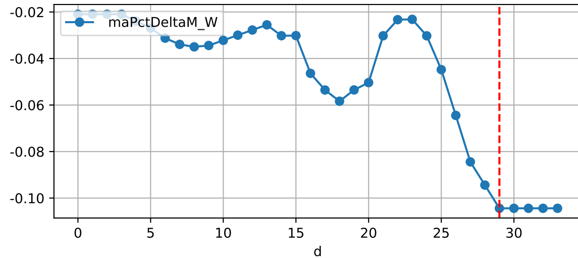
Daily %DeltaM and %DeltaM/1000ml ETcIdef for M_W (-10.4%/D, -6.6%/1000ml ET)
