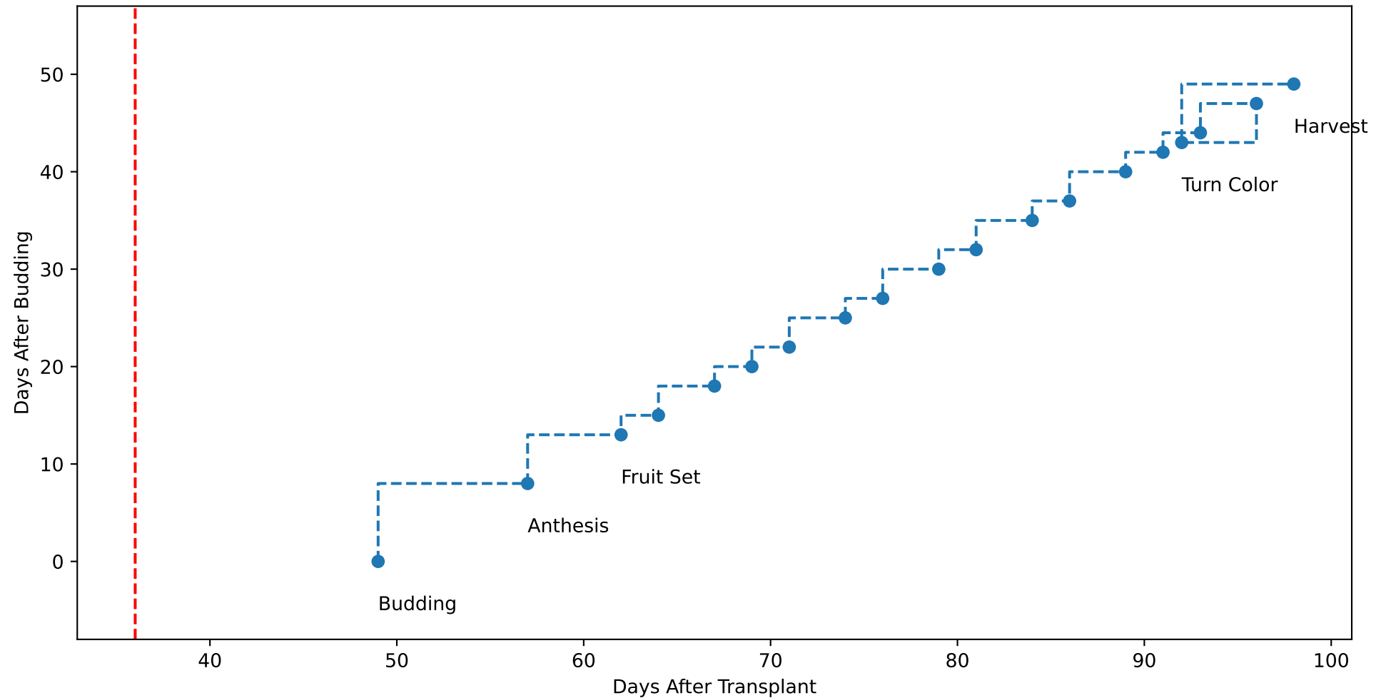
G3-8 TsN6 (plot by adjDAT)
