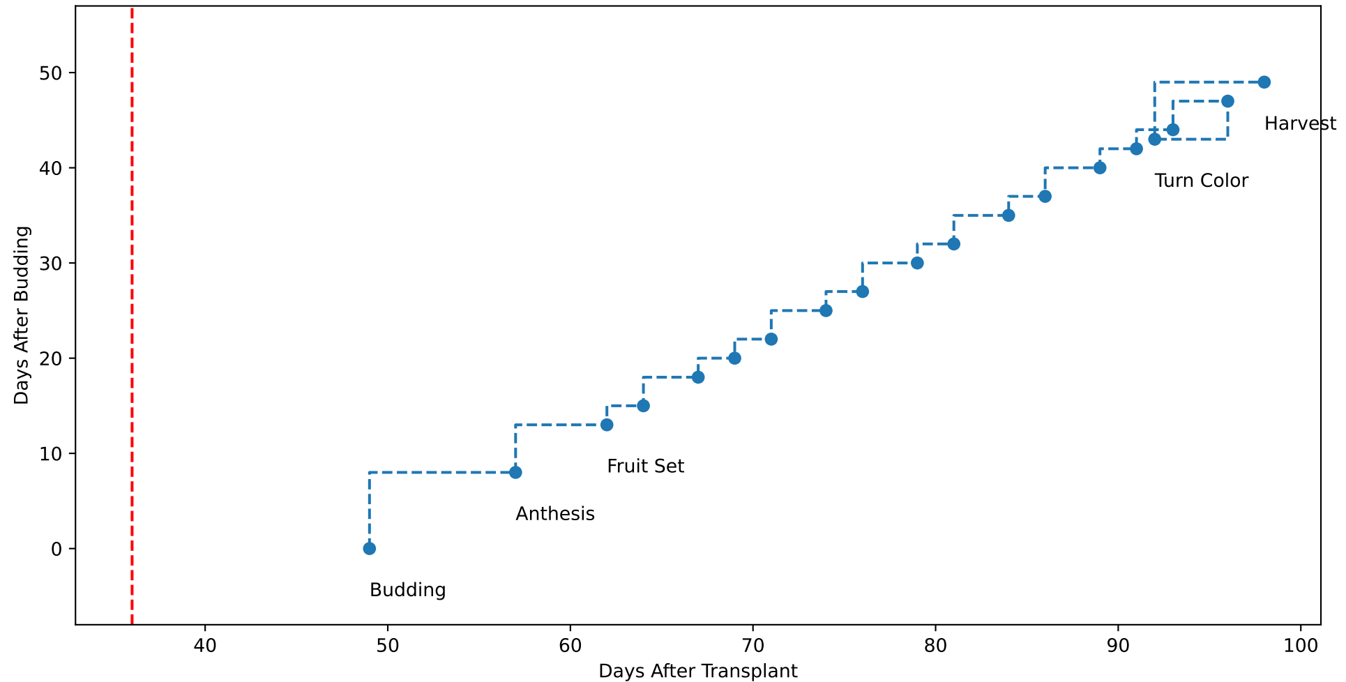
G3-8 TsN6 (plot by DAT)
