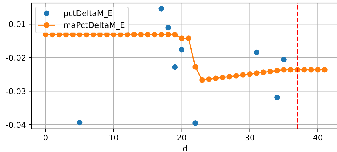
Daily %DeltaM and %DeltaM/1000ml ETcldef for M_E (-2.4%/D, -2.4%/1000ml ET)
