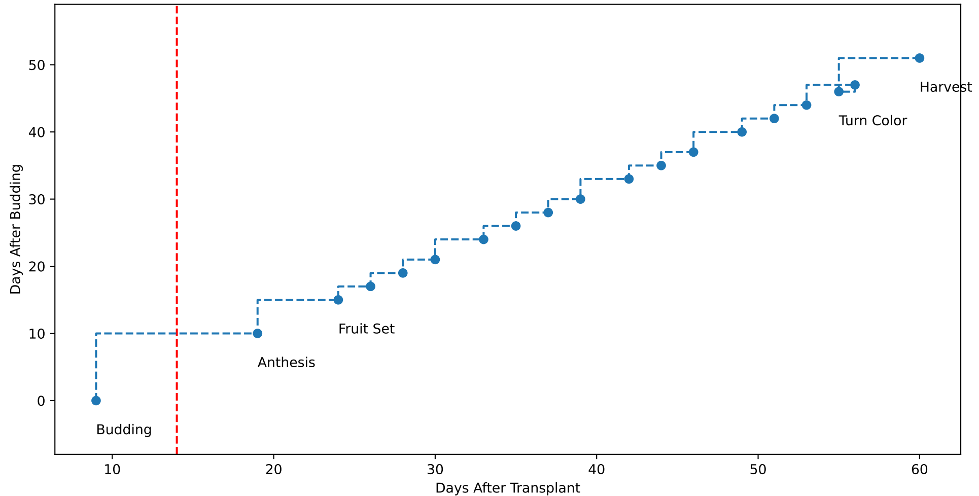
G3-9 TsN1 (plot by adjDAT)
