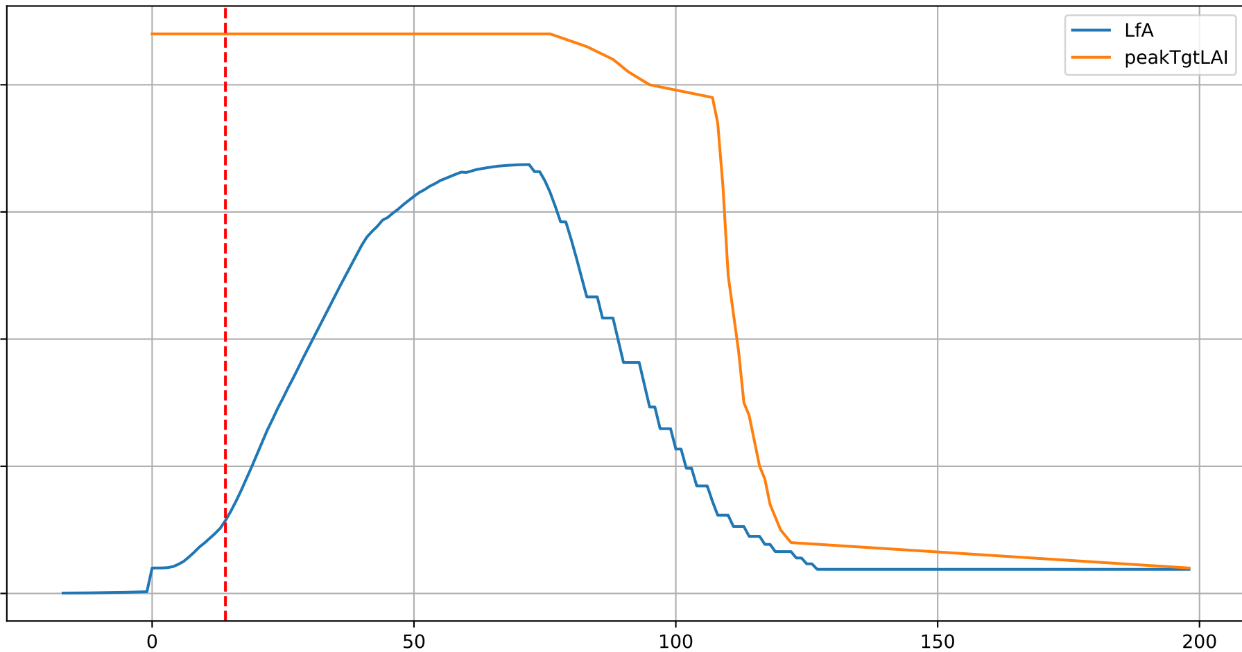
G3-9: ['LfA', 'peakTgtLAI']
