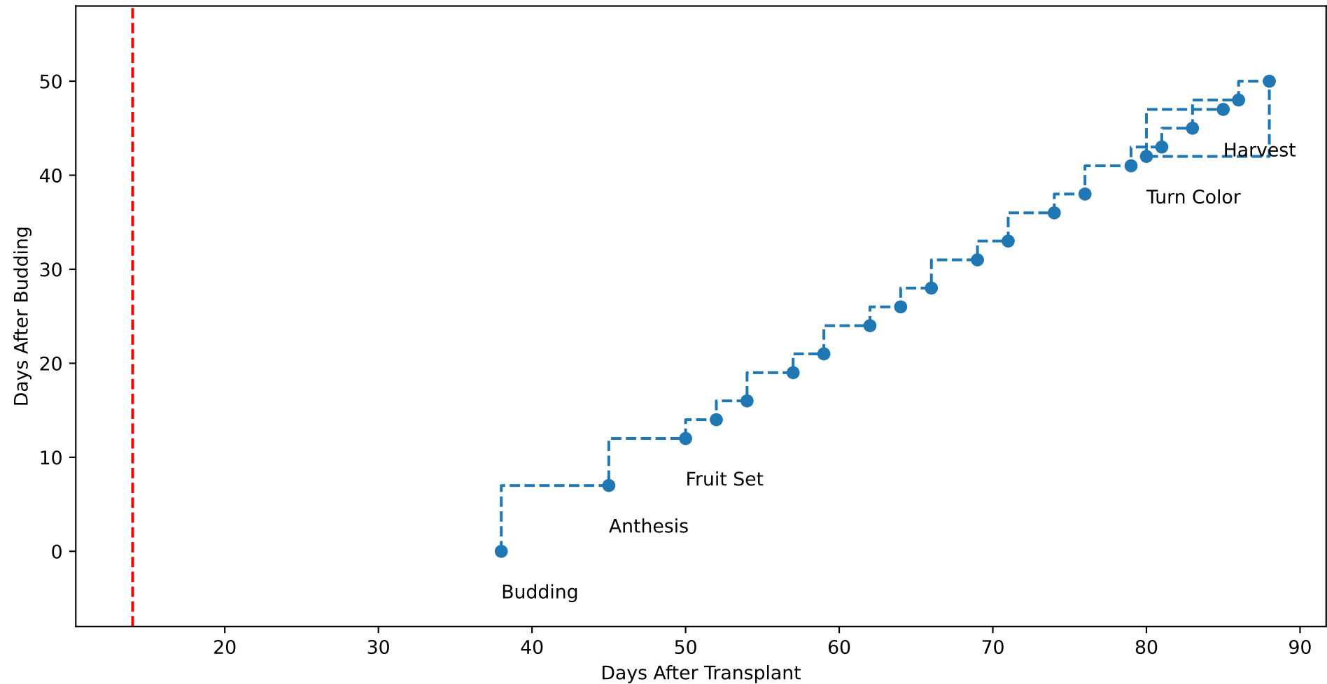
G3-9 TsN5 (plot by DAT)
