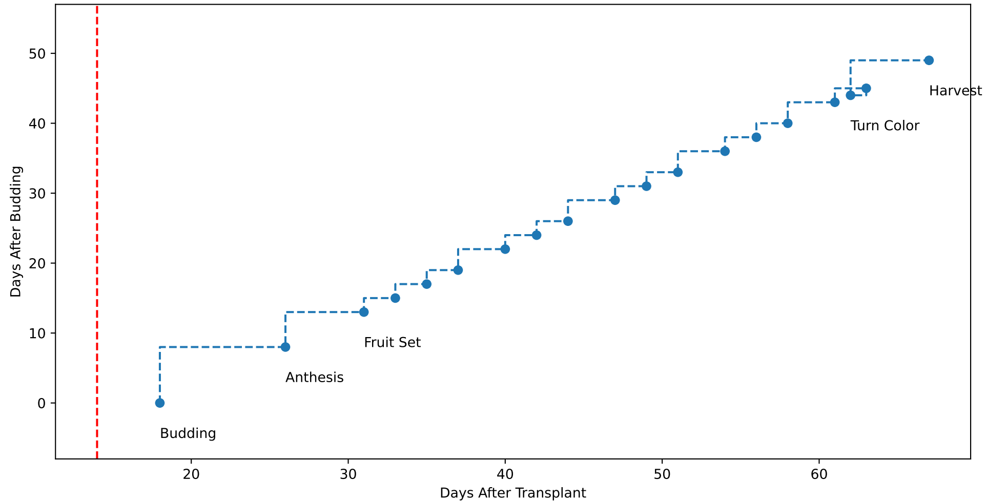
G3-9 TsN2 (plot by DAT)
