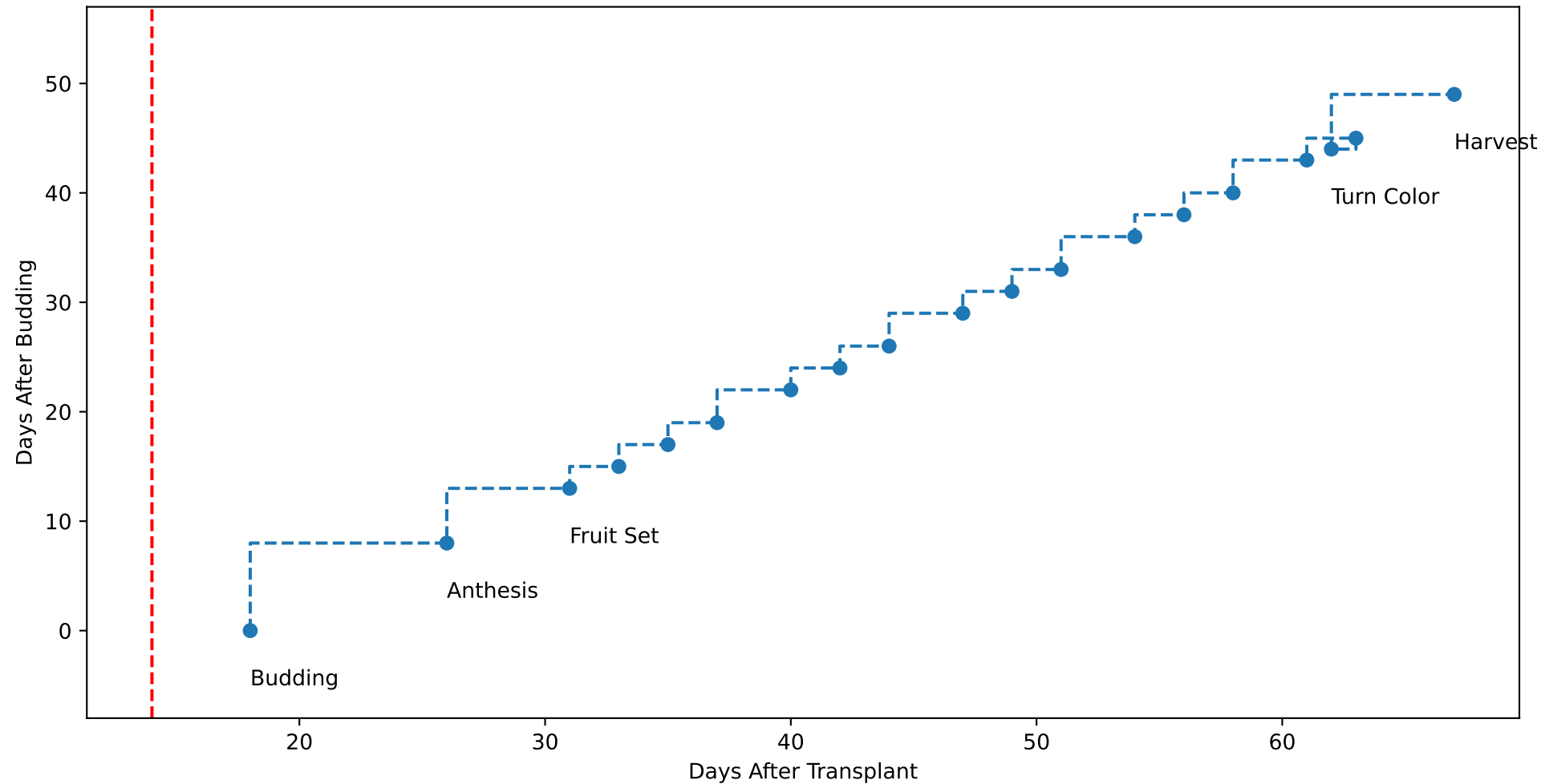
G3-9 TsN2 (plot by adjDAT)
