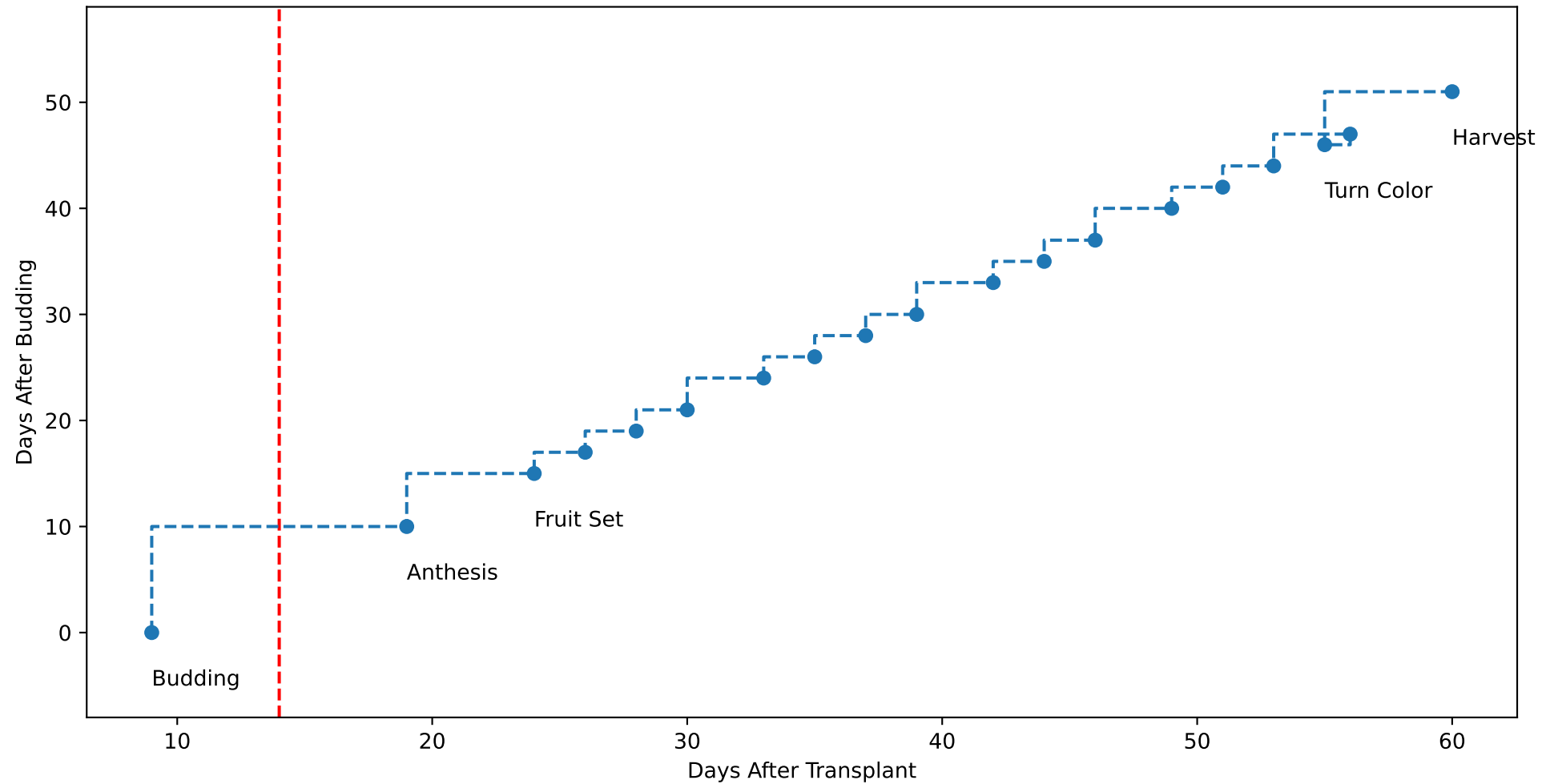
G3-9 TsN1 (plot by DAT)
