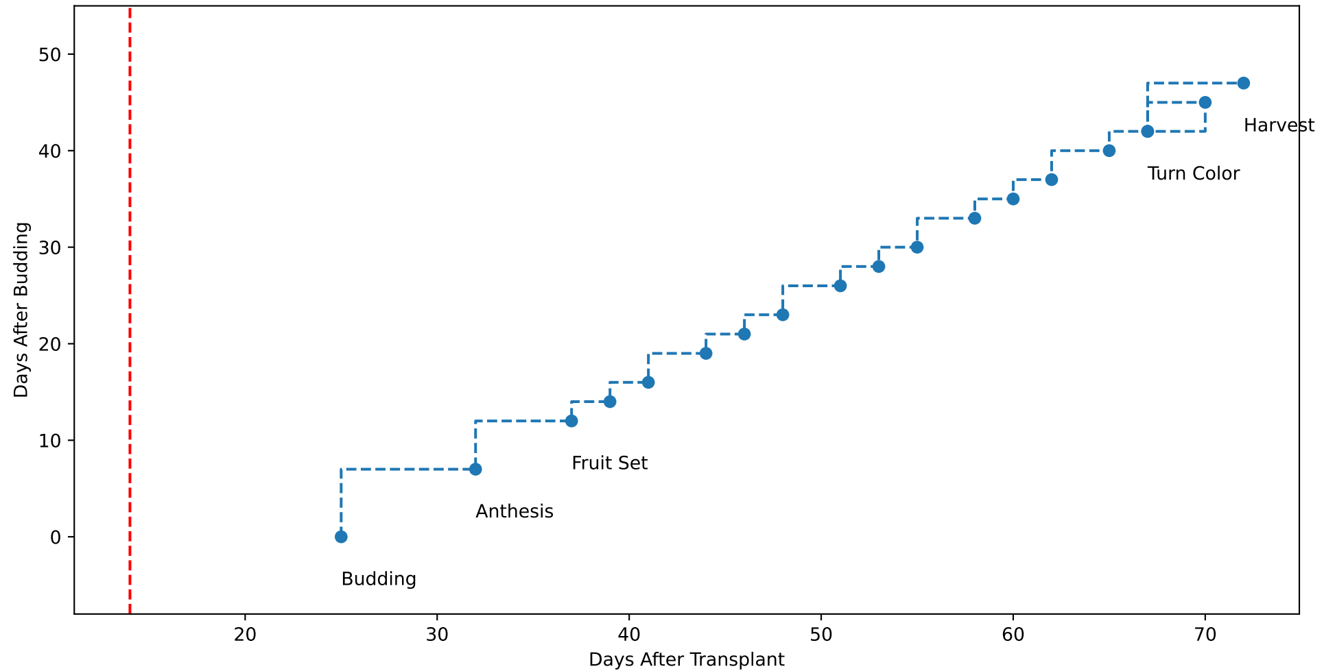
G3-9 TsN3 (plot by DAT)
