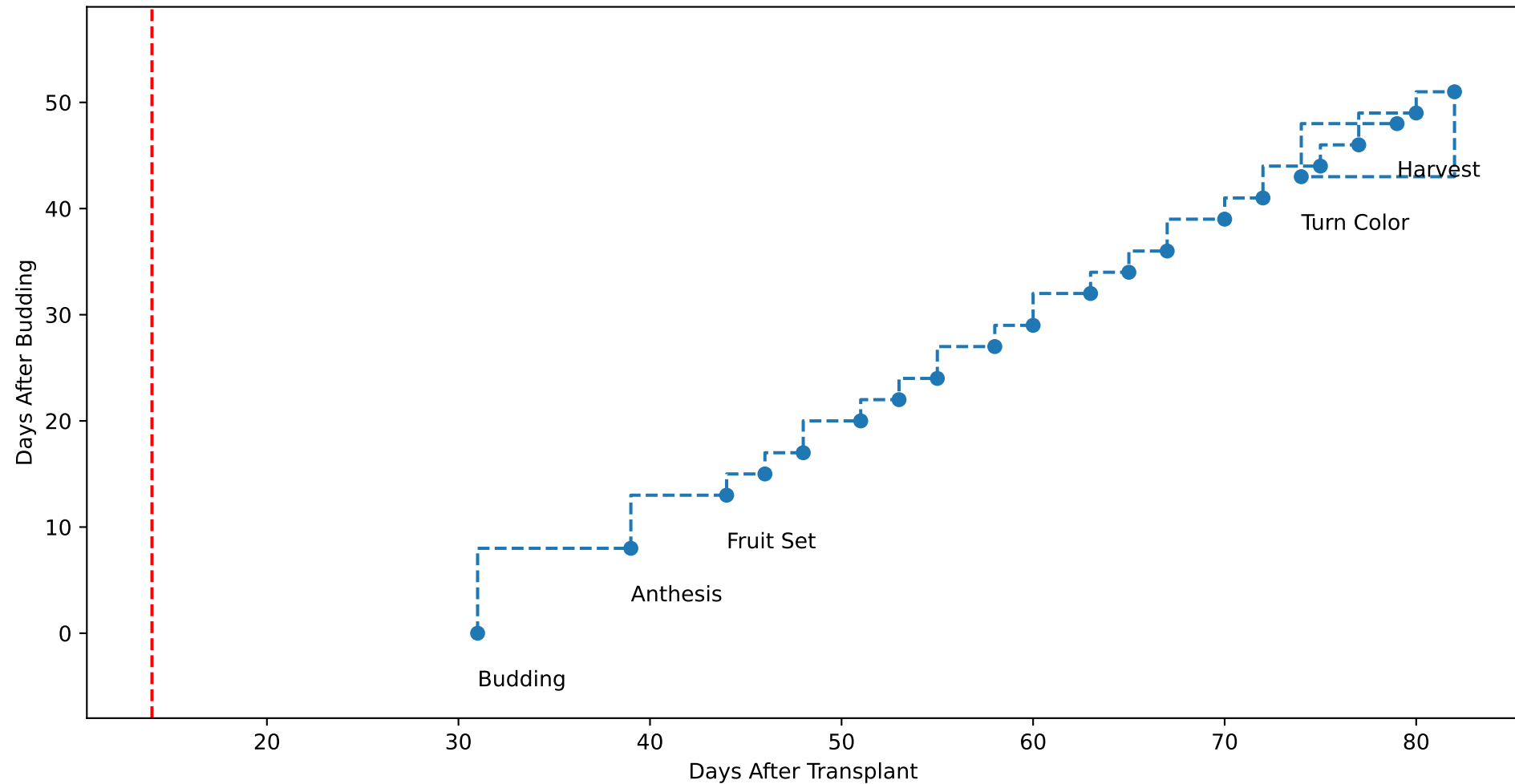
G3-9 TsN4 (plot by adjDAT)
