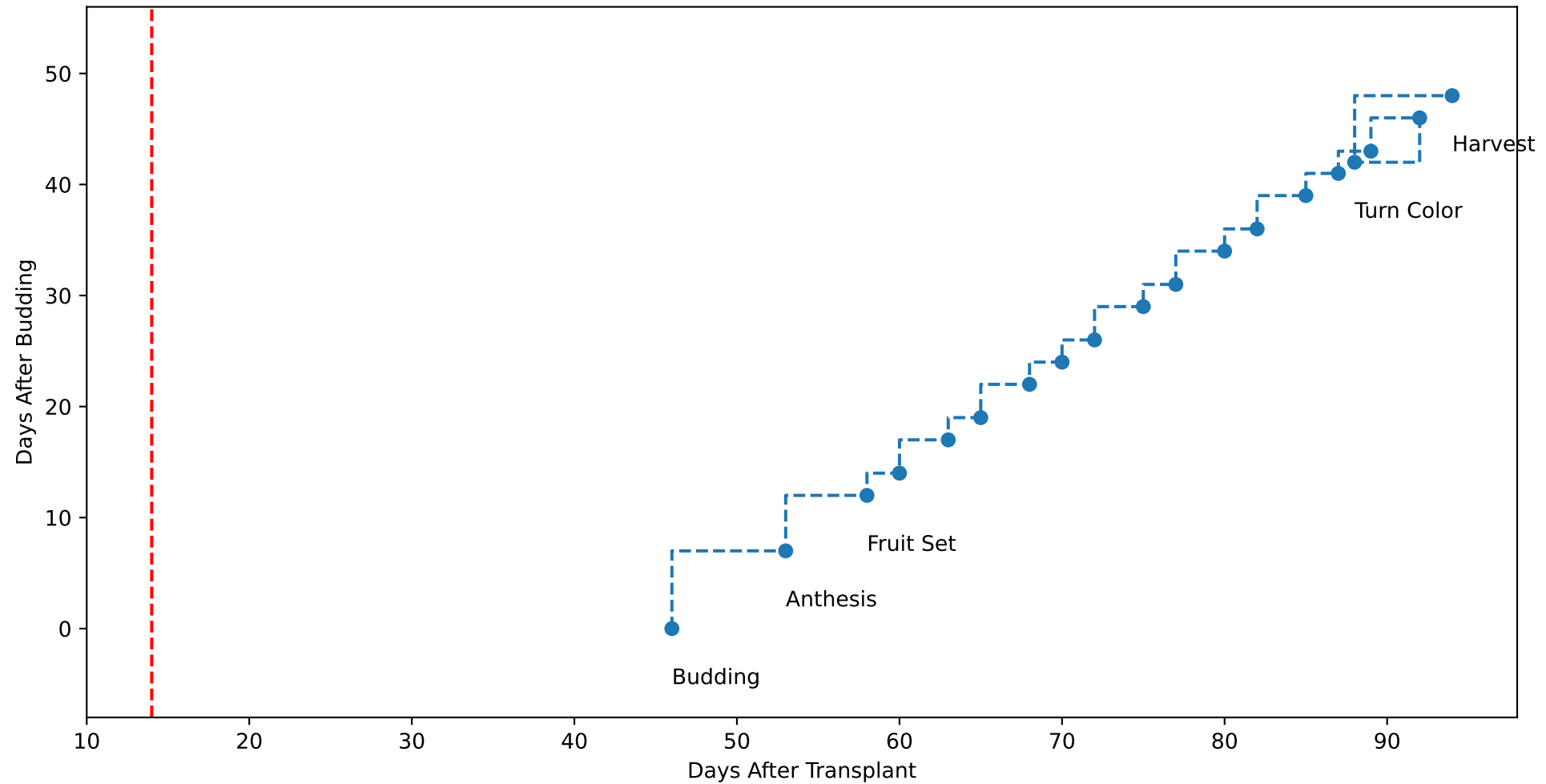
G3-9 TsN6 (plot by DAT)
