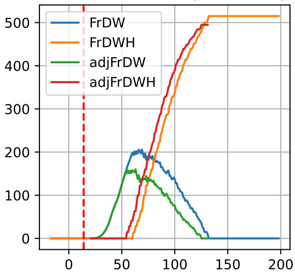
G3-9: ['FrDW', 'FrDWH', 'adjFrDW', 'adjFrDWH']
