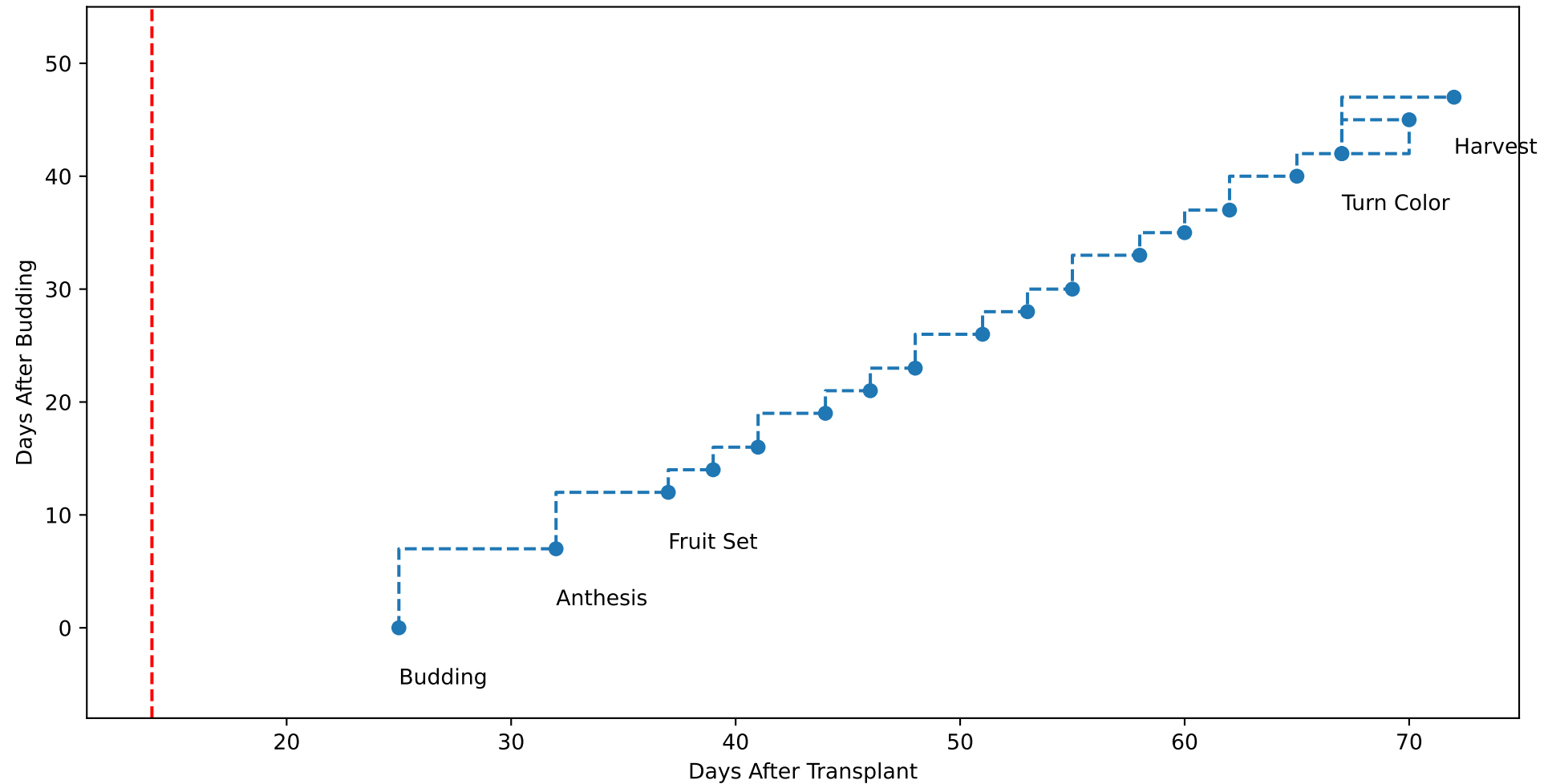
G3-9 TsN3 (plot by adjDAT)
