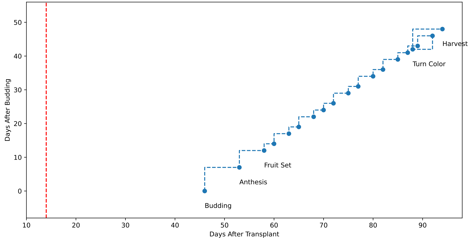
G3-9 TsN6 (plot by adjDAT)
