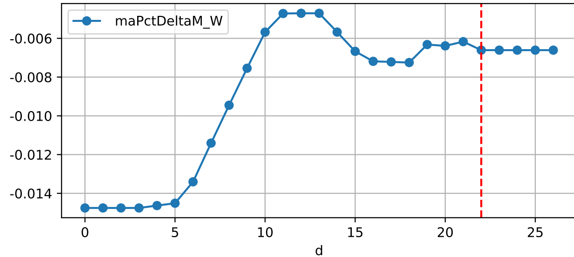
Daily %DeltaM and %DeltaM/1000ml ETcIdef for M_W (-0.7%/D, -0.6%/1000ml ET)
