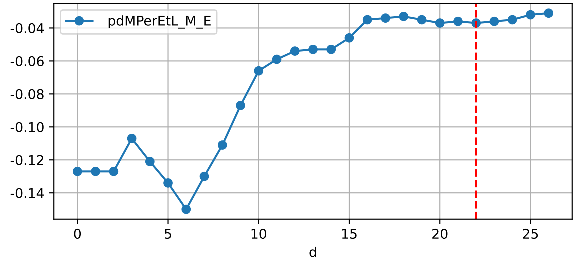
Daily %DeltaM and %DeltaM/1000ml ETcldef for M_E (-3.8%/D, -3.7%/1000ml ET)
