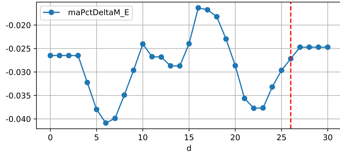
Daily %DeltaM and %DeltaM/1000ml ETcldef for M_E (-2.7%/D, -2.4%/1000ml ET)
