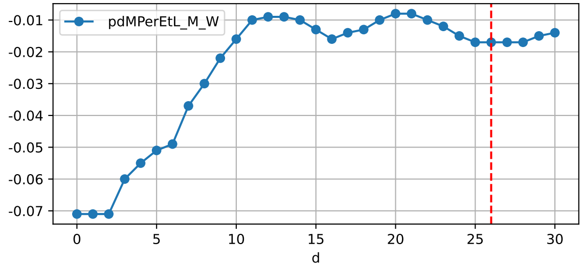
Daily %DeltaM and %DeltaM/1000ml ETcIdef for M_W (-2.0%/D, -1.7%/1000ml ET)
