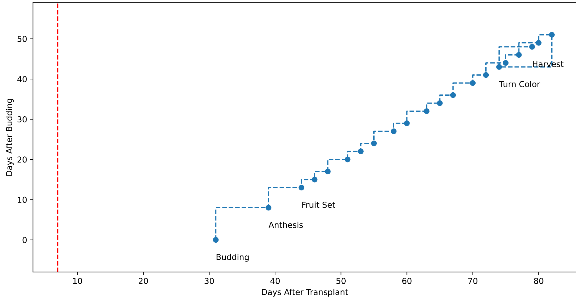
G3-9 TsN4 (plot by adjDAT)
