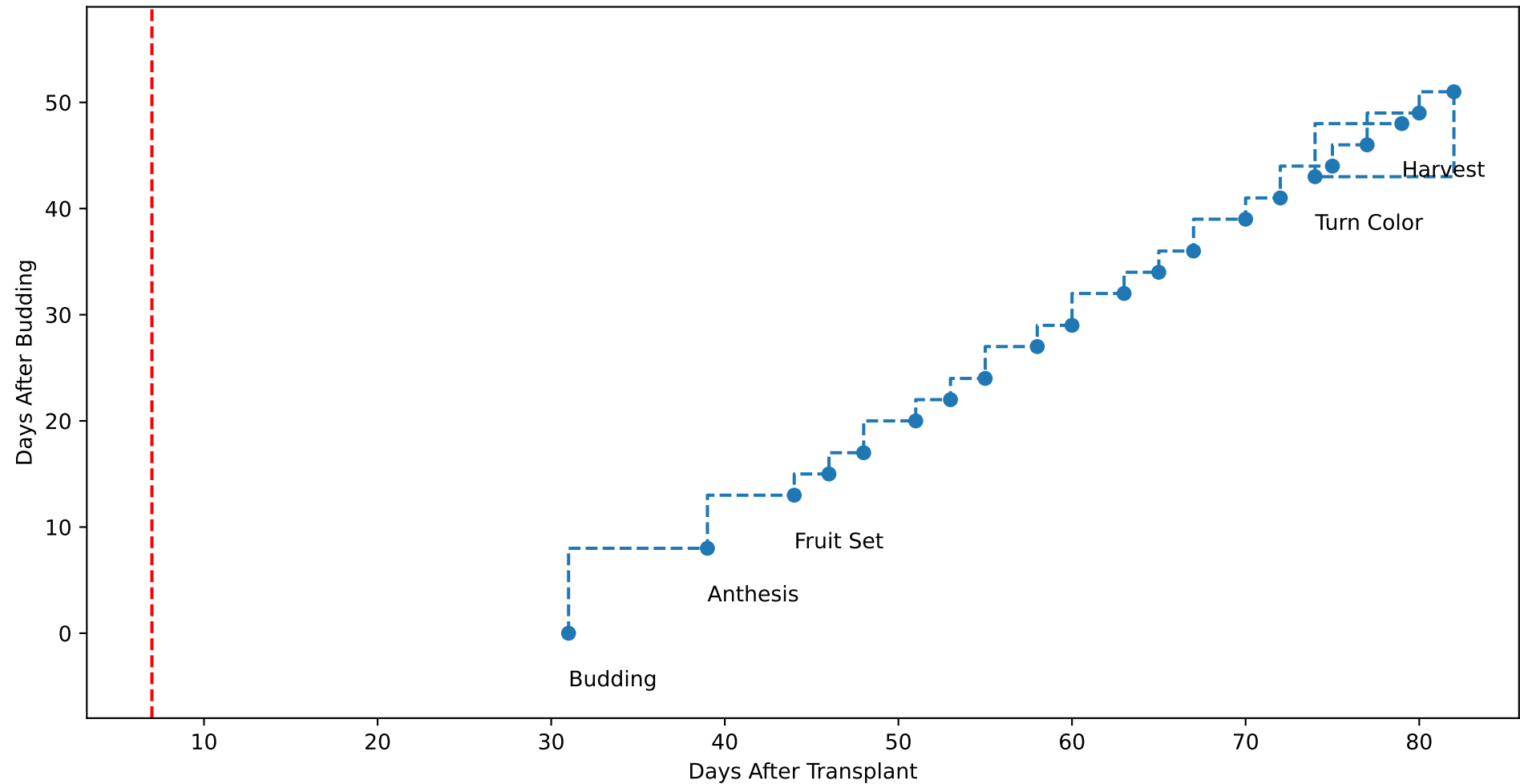
G3-9 TsN4 (plot by DAT)
