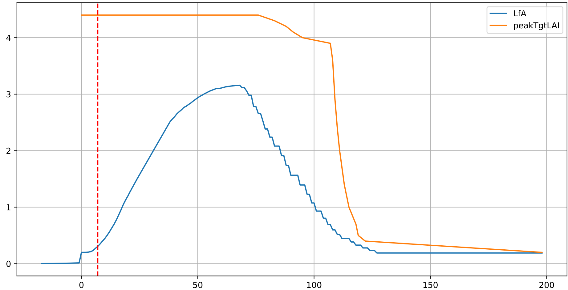
G3-9: ['LfA', 'peakTgtLAI']
