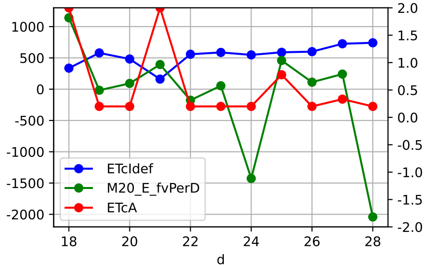
M20_E daily ETcldef vs estFv (avgPctDeltaM = -2.8%)
