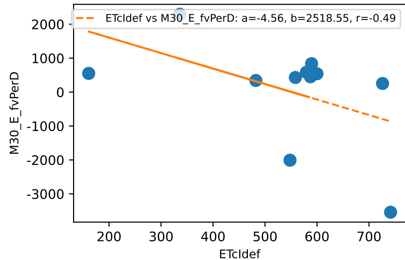
M30_E daily ETcldef vs estFv (avgPctDeltaM = -1.6%)
