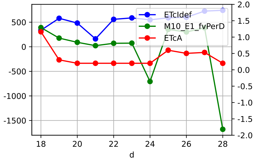
M10_E1 daily ETcldef vs estFv (avgPctDeltaM = -6.7%)
