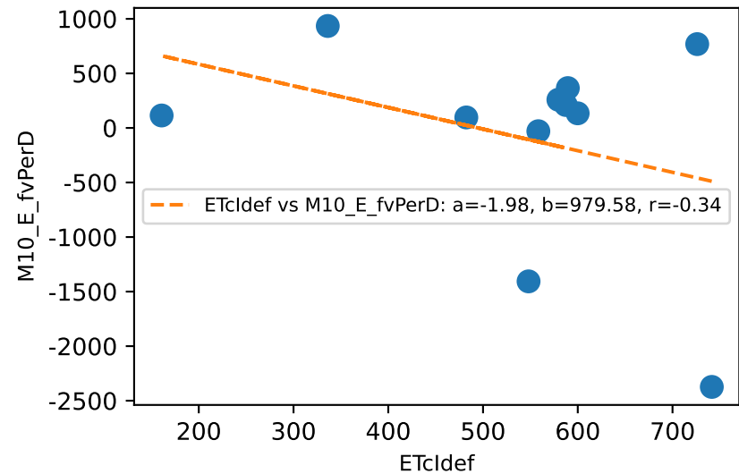
M10_E daily ETcldef vs estFv (avgPctDeltaM = -1.5%)
