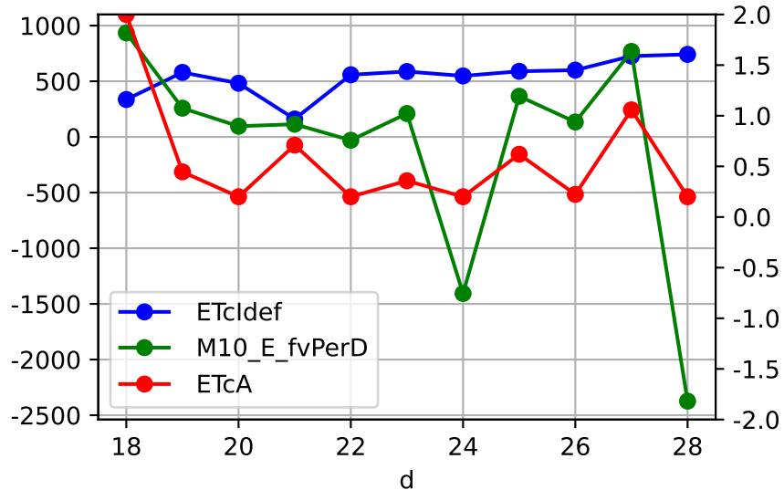
M10_E daily ETcldef vs estFv (avgPctDeltaM = -1.5%)
