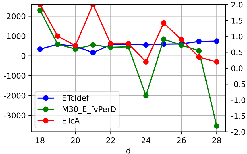
M30_E daily ETcldef vs estFv (avgPctDeltaM = -1.6%)
