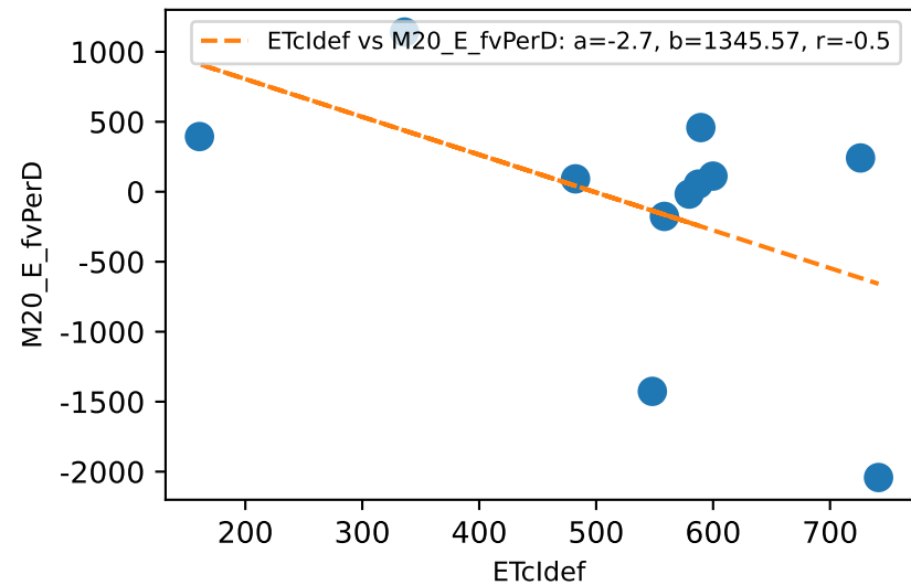
M20_E daily ETcldef vs estFv (avgPctDeltaM = -2.8%)
