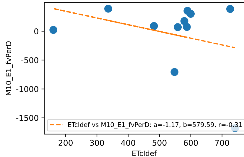
M10_E1 daily ETcldef vs estFv (avgPctDeltaM = -6.7%)
