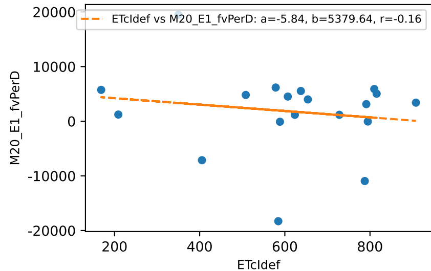
M20_E1 daily ETcldef vs estFv (avgPctDeltaM = -2.8%)
