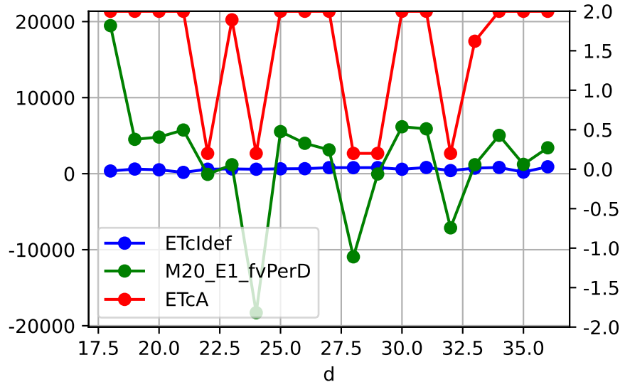
M20_E1 daily ETcldef vs estFv (avgPctDeltaM = -2.8%)
