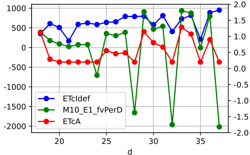
M10_E1 daily ETcldef vs estFv (avgPctDeltaM = -6.5%)
