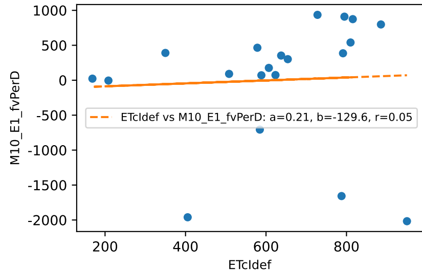
M10_E1 daily ETcldef vs estFv (avgPctDeltaM = -6.5%)
