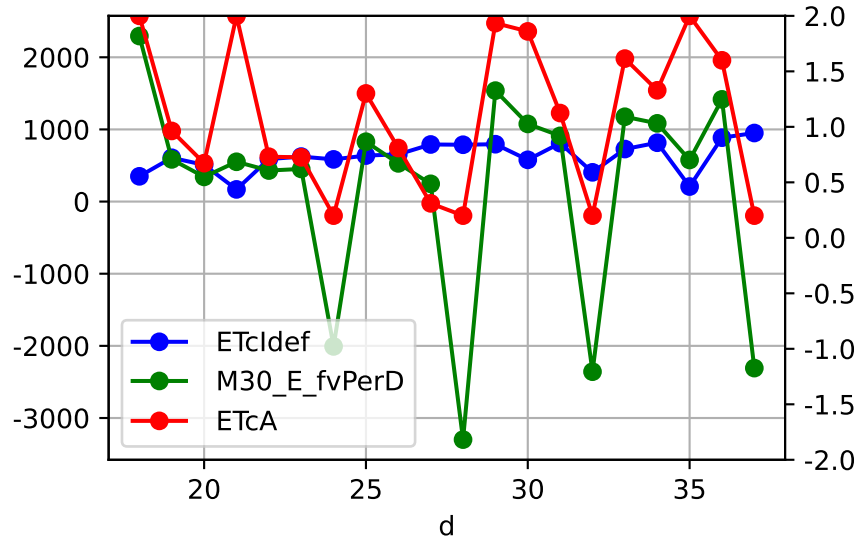
M30_E daily ETcldef vs estFv (avgPctDeltaM = -3.7%)
