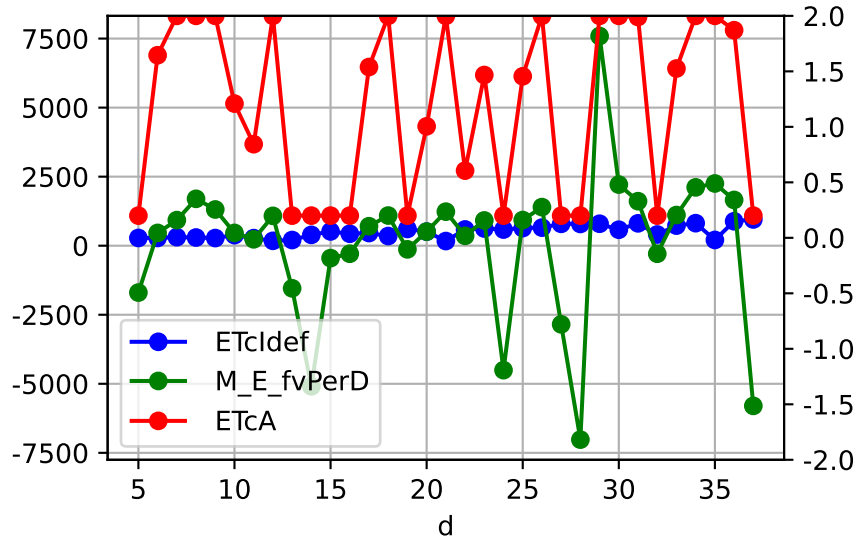
M_E daily ETcldef vs estFv (avgPctDeltaM = -2.4%)
