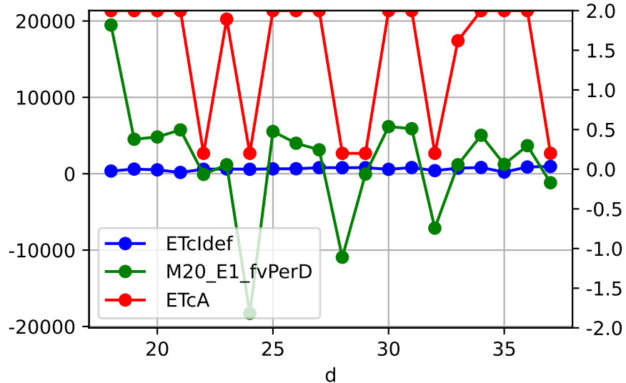
M20_E1 daily ETcldef vs estFv (avgPctDeltaM = -3.0%)
