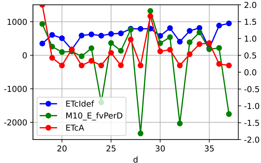
M10_E daily ETcldef vs estFv (avgPctDeltaM = -3.4%)
