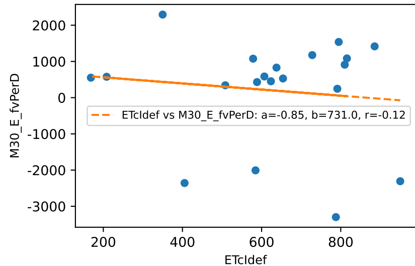
M30_E daily ETcldef vs estFv (avgPctDeltaM = -3.7%)
