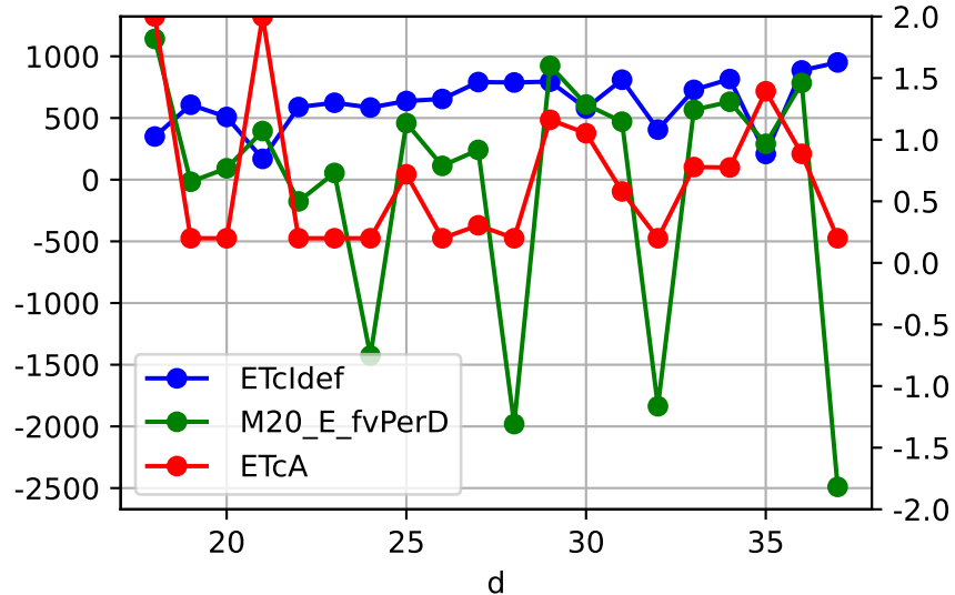
M20_E daily ETcldef vs estFv (avgPctDeltaM = -4.6%)
