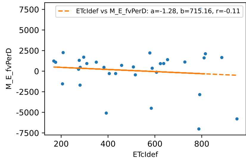
M_E daily ETcldef vs estFv (avgPctDeltaM = -2.4%)
