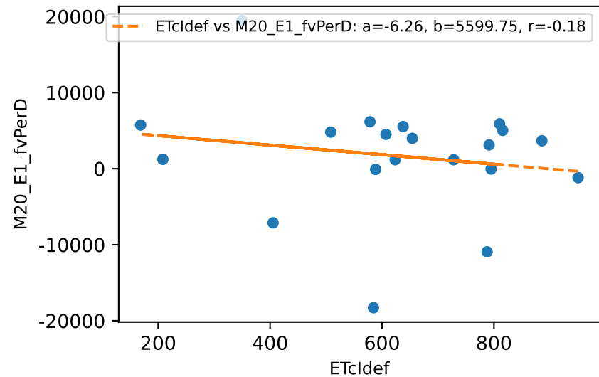
M20_E1 daily ETcldef vs estFv (avgPctDeltaM = -3.0%)
