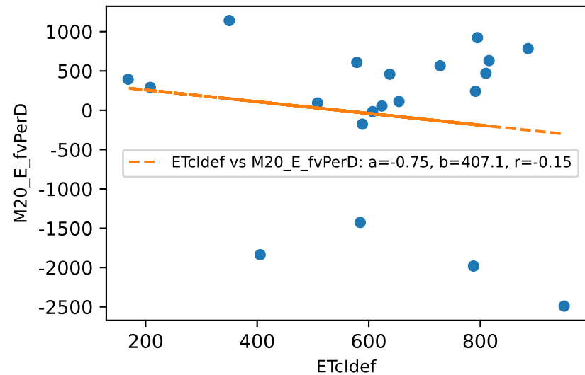
M20_E daily ETcldef vs estFv (avgPctDeltaM = -4.6%)
