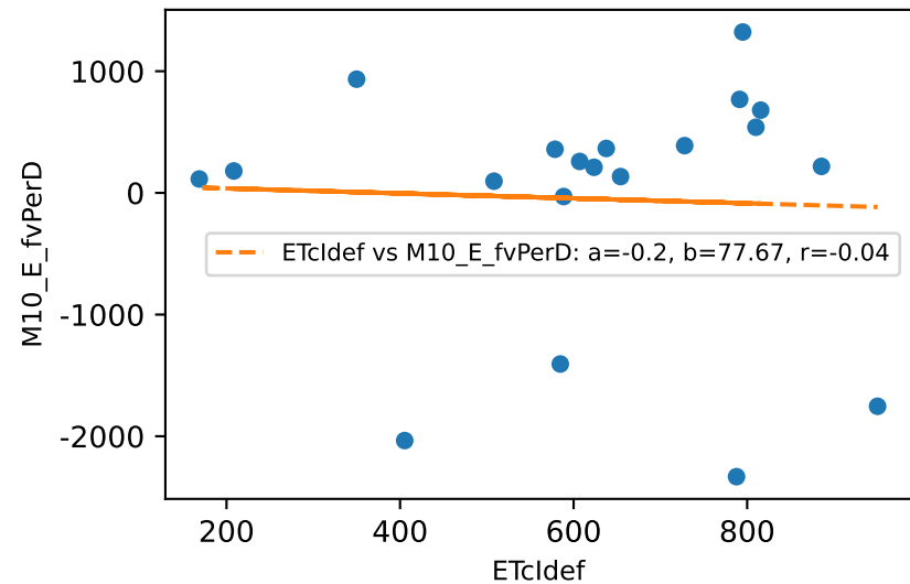
M10_E daily ETcldef vs estFv (avgPctDeltaM = -3.4%)
