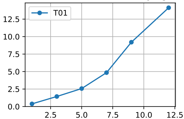
FrV (P10AE-063-19) Plot By Age
