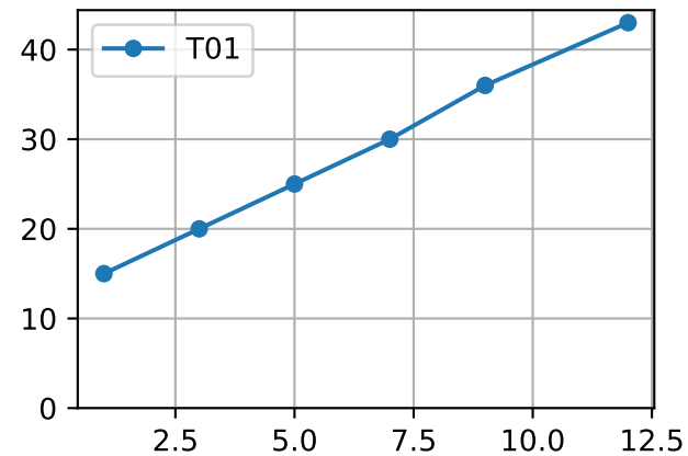
FrD (P10AE-076-5) Plot By Age
