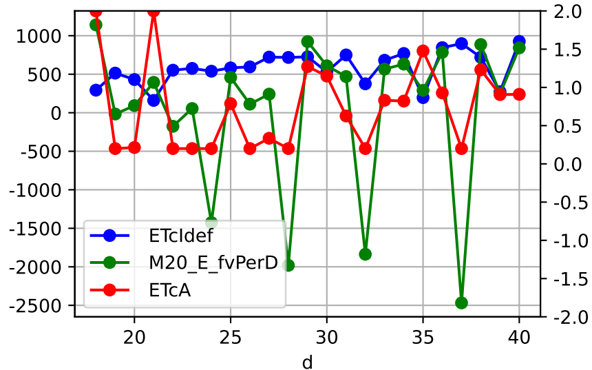
M20_E daily ETcldef vs estFv (avgPctDeltaM = -6.3%)
