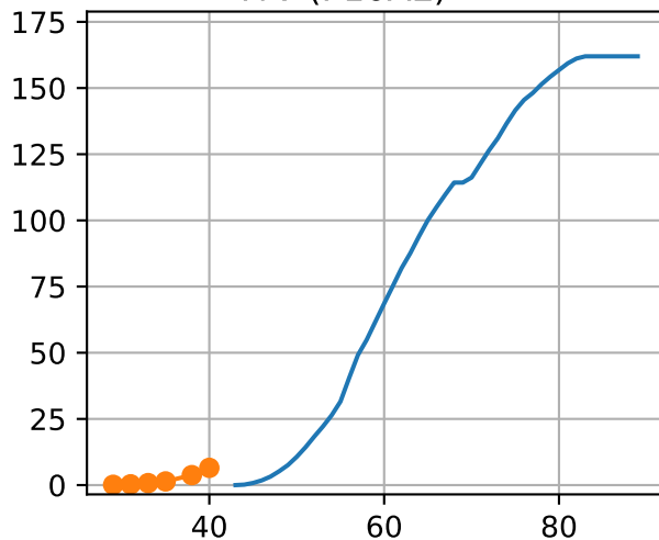
FrV(['S1T1Fr5'])
