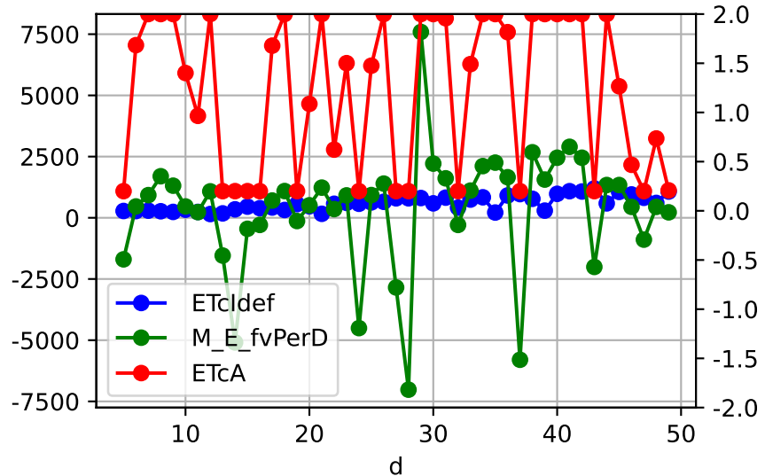
M_E daily ETcldef vs estFv (avgPctDeltaM = -4.4%)
