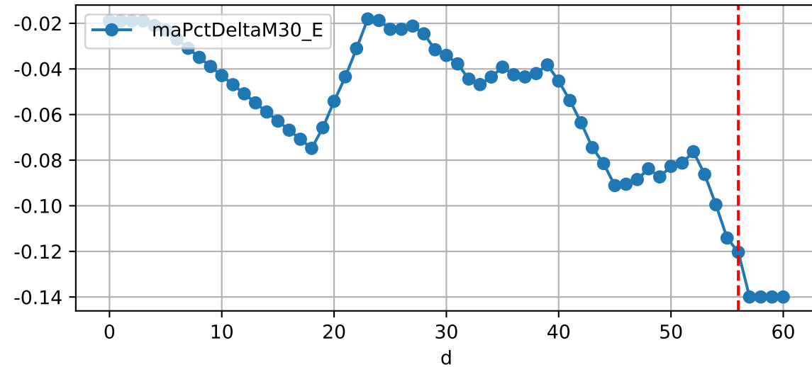
Daily %DeltaM and %DeltaM/1000ml ETcIdef for M30_E (-12.0%/D, -12.7%/1000ml ET)
