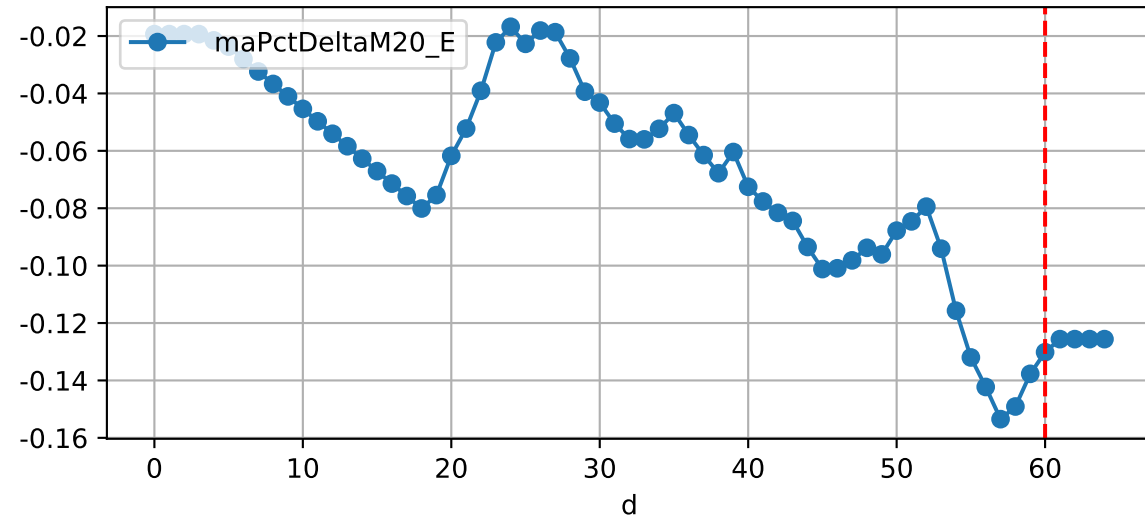
Daily %DeltaM and %DeltaM/1000ml ETcIdef for M20_E (-13.0%/D, -12.3%/1000ml ET)
