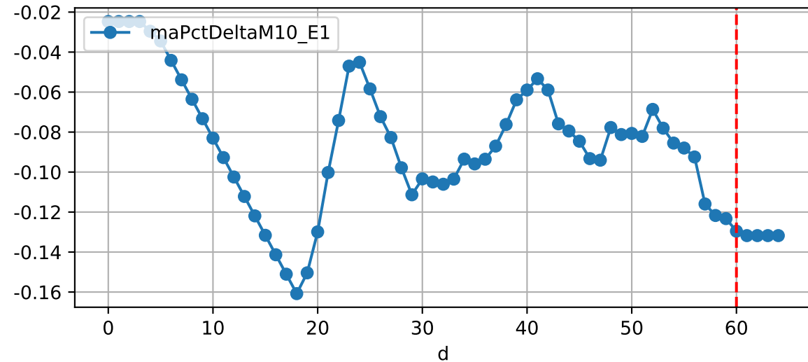
Daily %DeltaM and %DeltaM/1000ml ETcldef for M10_E1 (-13.0%/D, -12.2%/1000ml ET)
