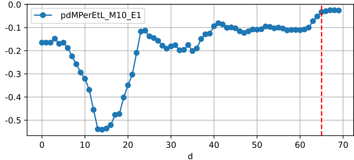
Daily %DeltaM and %DeltaM/1000ml ETcldef for M10_E1 (-3.0%/D, -3.3%/1000ml ET)
