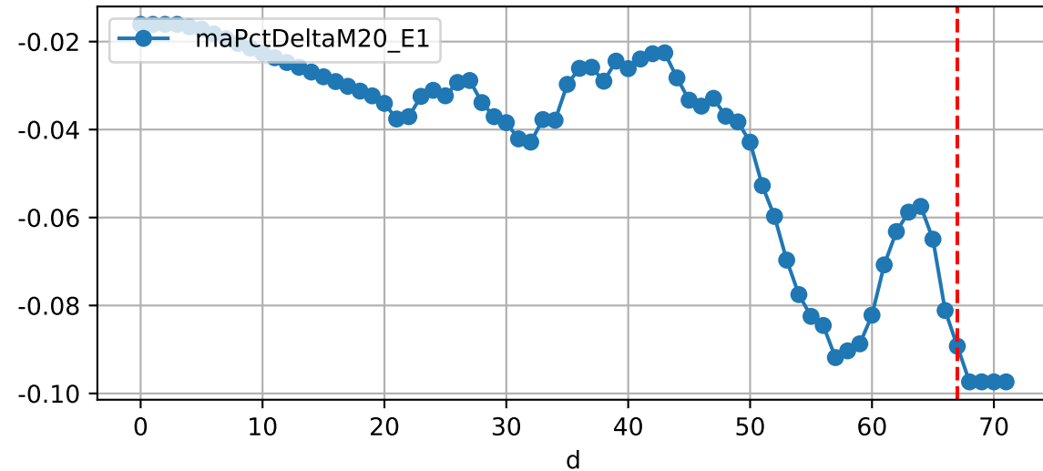
Daily %DeltaM and %DeltaM/1000ml ETcldef for M20_E1 (-8.9%/D, -7.3%/1000ml ET)
