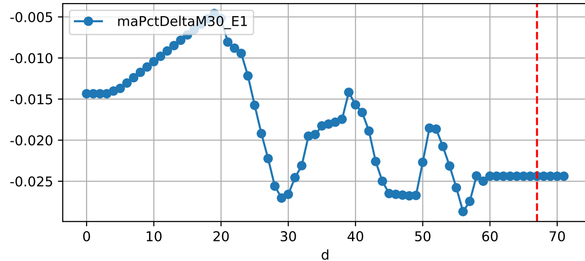
Daily %DeltaM and %DeltaM/1000ml ETcldef for M30_E1 (-2.4%/D, -2.0%/1000ml ET)
