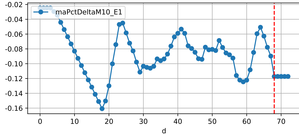
Daily %DeltaM and %DeltaM/1000ml ETcIdef for M10_E1 (-11.7%/D, -8.5%/1000ml ET)
