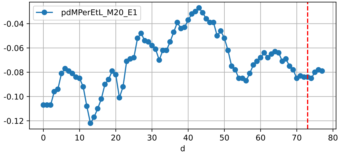
Daily %DeltaM and %DeltaM/1000ml ETcIdef for M20_E1 (-11.4%/D, -8.4%/1000ml ET)
