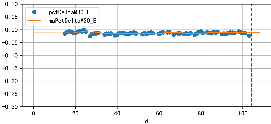
Daily %DeltaM and %DeltaM/1000ml ETcIdef for M30_E (-1.2%/D, -2.5%/1000ml ET)
