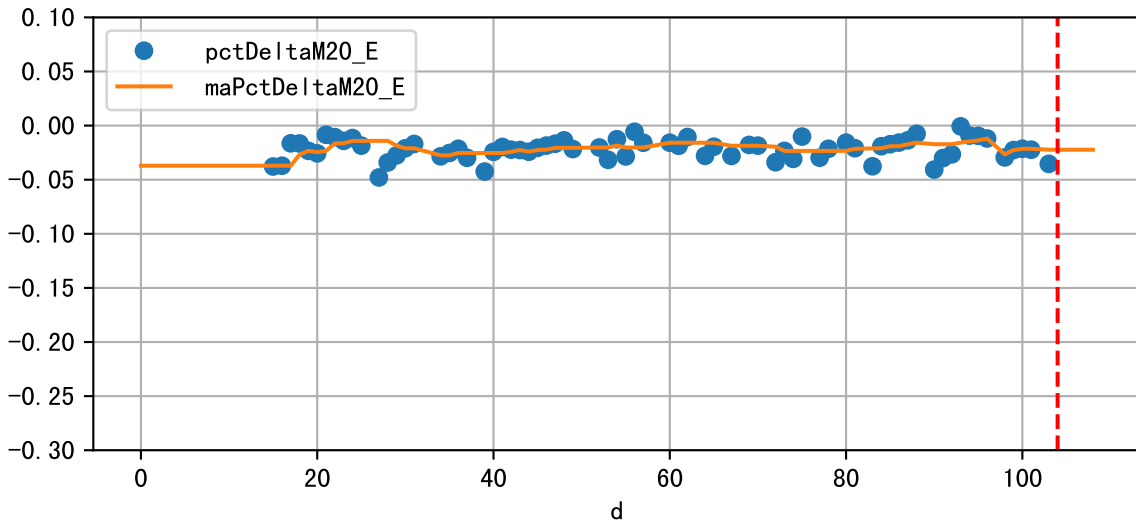
Daily %DeltaM and %DeltaM/1000ml ETcIdef for M20_E (-2.2%/D, -4.5%/1000ml ET)
