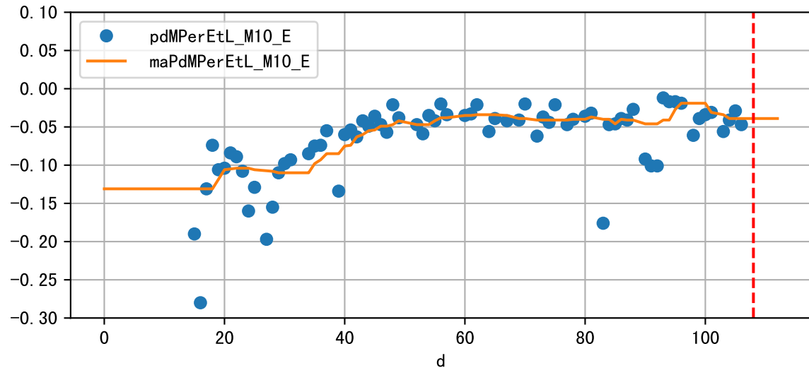
Daily %DeltaM and %DeltaM/1000ml ETcIdef for M10_E (-1.7%/D, -3.9%/1000ml ET)
