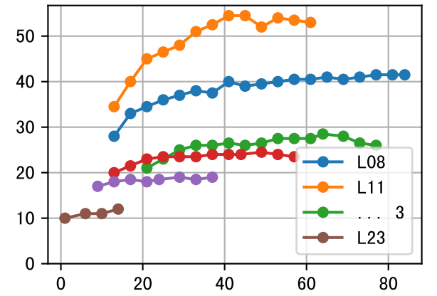
LfW (P10AE-087-27) Plot By Age
