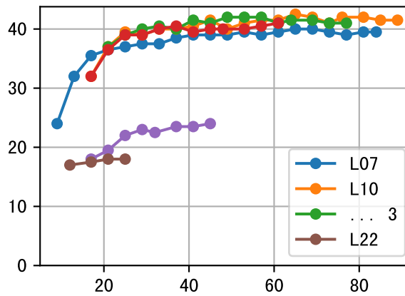
P10AE (Raw data plots) LfL (P10AE-114-7) Plot By Age
