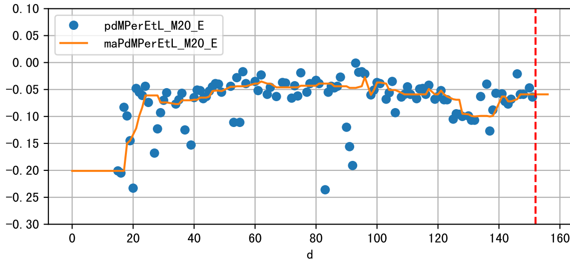
Daily %DeltaM and %DeltaM/1000ml ETcIdef for M20_E (-4.4%/D, -5.9%/1000ml ET)
